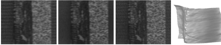
Fig. 6. First and second from the left: input images of the first data set. The two images are both defocused and motion-blurred. Motion blurring is caused by a sideways motion of the camera. Third from the left: recovered radiance. Fourth from the left: recovered depth map.
