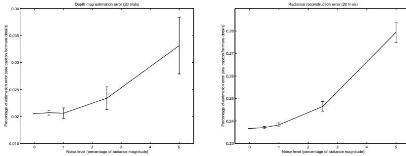
Fig. 5. Left: depth map estimation for 5 levels of additive Gaussian noise. The plot shows the error bar for 20 trials with a staircase depth map and a random radiance. We compute the RMS error between the estimated depth and the true depth, and normalize it with respect to the norm of the true depth (see eq. (24)). Right: radiance estimation for 5 levels of additive Gaussian noise. As in the previous error bar, we compute the RMS error between the true radiance and the reconstructed radiance and then normalize it with respect to the norm of the true radiance.
