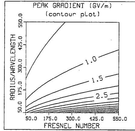
Figure 1: E_a vs. \{N, a/\lambda\} @ \lambda = 1\mu\text{m}, E_e = 10\text{GV/m} .
