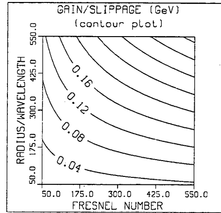
Figure 2: \Delta W_s vs. \{N, a/\lambda\} @ \lambda = 1\mu\text{m}, E_e = 10\text{GV/m} .
