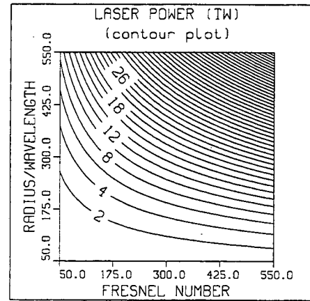
Figure 3: P_0 vs. \{N, a/\lambda\} @ \lambda = 1\mu\text{m}, E_e = 10\text{GV/m} .
