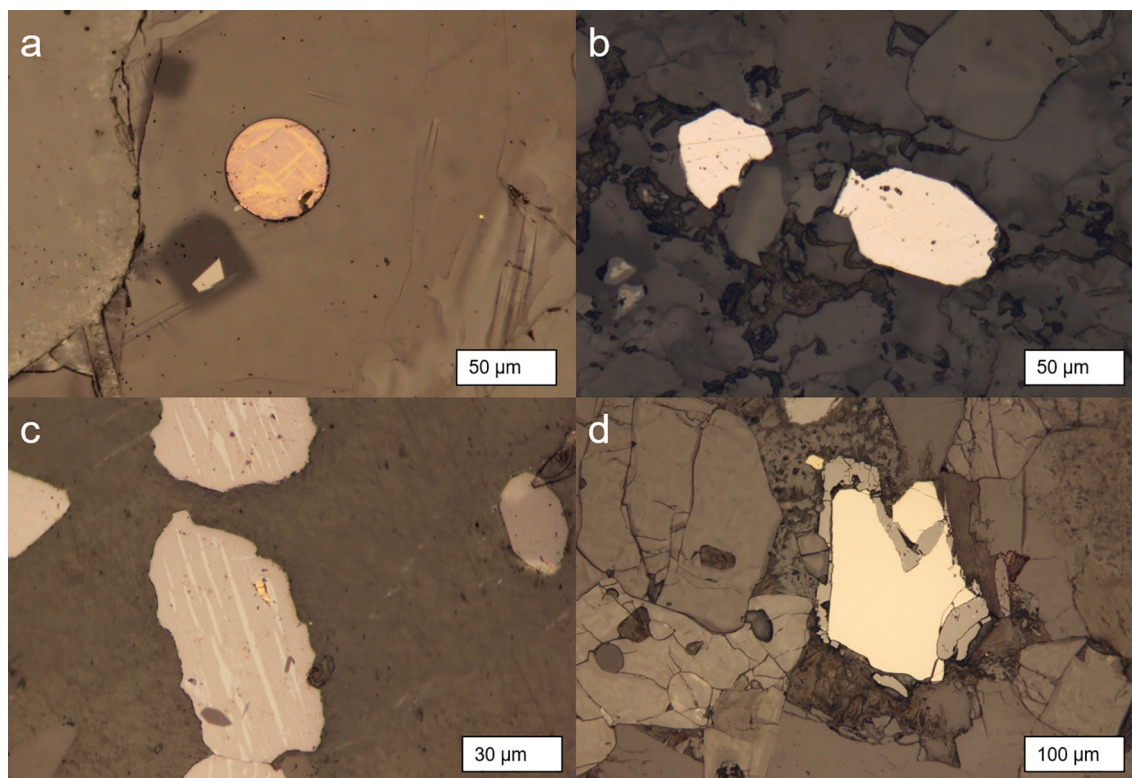
Fig. 1. Photomicrographs of sulfides targeted for laser ablation analysis. (A) Immiscible sulfide bleb from the Kilauea Iki lava lake (KI67-3-76.2) showing needle-like exsolution textures. A second minute ( \leq 1 \mu\text{m} diameter) sulfide is visible on the right. (B) Pyrite from the Archean Superior province tonalite (WXP99-119). (C) Small chalcopyrite inclusion (yellow) hosted in magnetite having ilmenite exsolution from a Mesozoic granite (10RMG005). (D) Pyrite rimmed by magnetite from the Paleozoic Ellicott City Granodiorite (AG1401). (For interpretation of the references to color in this figure legend, the reader is referred to the web version of this article.)
