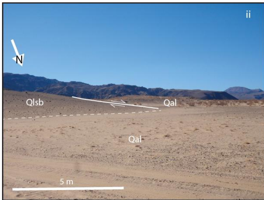
Figure 4.2, cont. (B-E) Field photographs of proximal Last Chance range front, displaying evidence for prevalent regional normal faulting. See Fig. 4.1B for locations.
