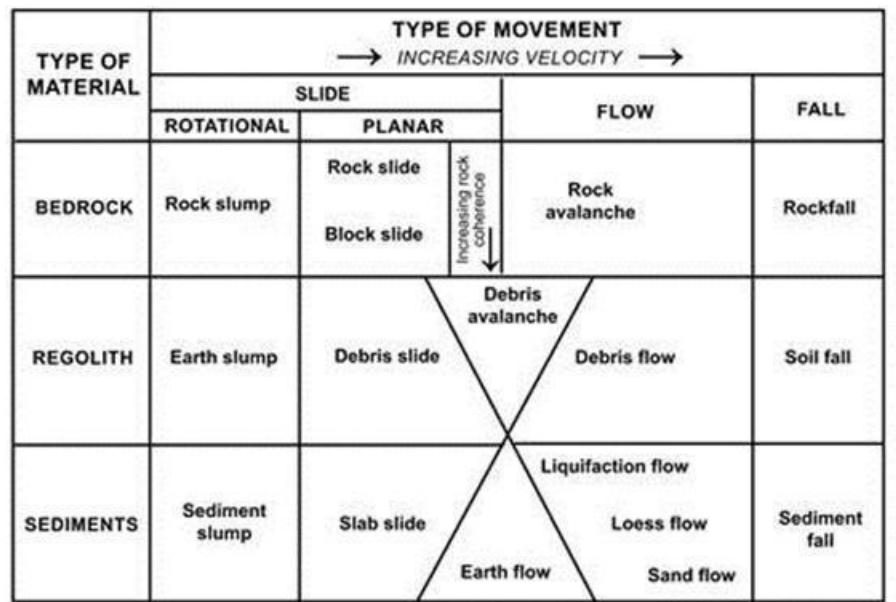
Figure 1.3. Classification of mass movements based on type of material and type of movement (after Malin, 1992).
