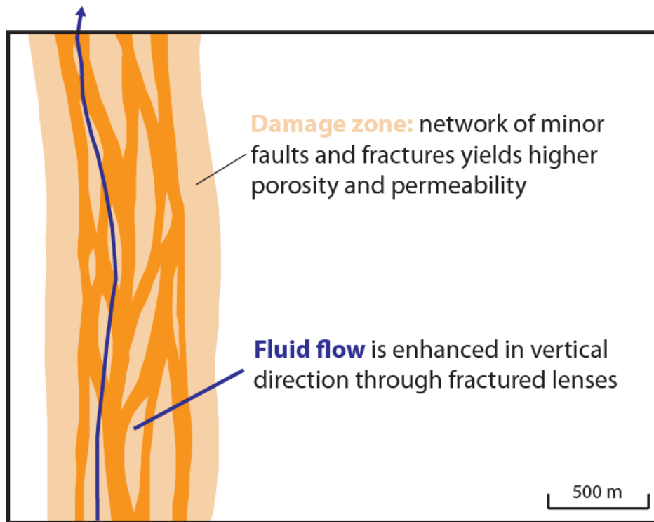
Figure 5.14. Schematic cross section through a vertical fault zone (Carboneras in southeast Spain; after Faulkner and Rutter, 2001). Brittle fault zones can act as conduits for flow to the surface in the vertical direction through a network of subsidiary structures (e.g., minor faults and fractures) in the damage zone which yield high porosity and permeability.
