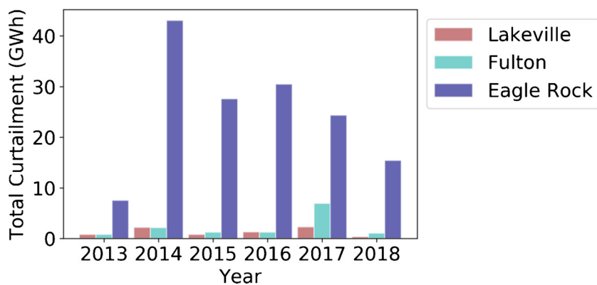
Fig. 12. Curtailment per year for power plants grouped by transmission lines at The Geysers (See Fig. 5 and Table 1 for grouping of power plants with transmission lines). Note that for all years except for 2013 and 2017, over 90 % of curtailment occurred at power plants linked to the lower capacity 115 KV Eagle Rock transmission line.
