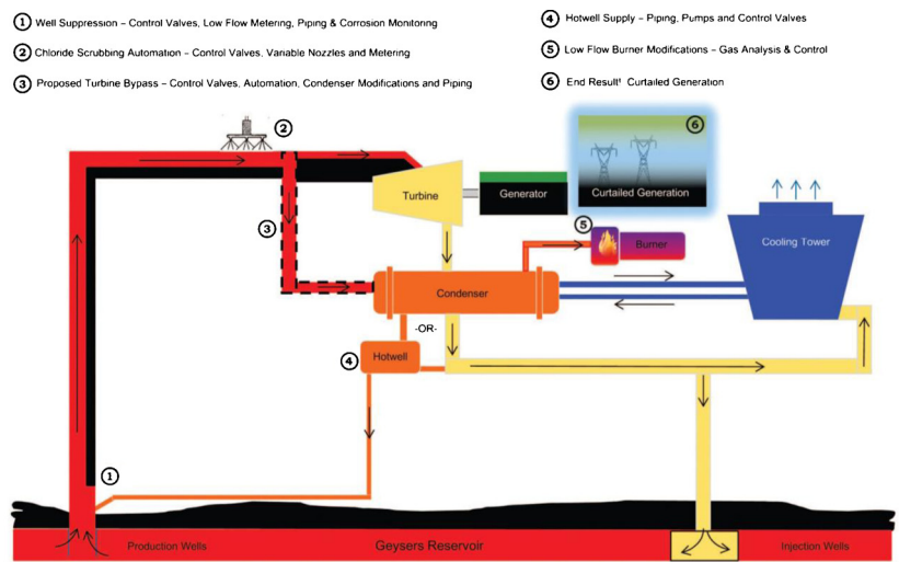
Fig. 17. Existing and proposed modifications to field operations at The Geysers to respond to curtailment (from Urbank and Jorgensen, 2016).
