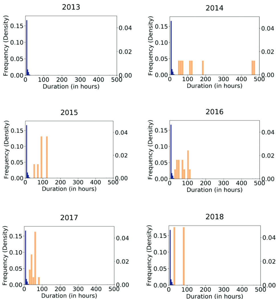
Fig. 9. The frequency distribution of the duration of curtailment events (grouped in 5-h bins) at The Geysers from 2013 to 2018. To facilitate viewing of the long-duration, low-frequency events, the data are plotted using a wider range of frequencies for the events spanning 1-25 h in length (plotted in blue, with the axis on the left), and a narrower range of frequencies for events greater than 25 h in length (plotted in orange, corresponding to the axis on the right) (For interpretation of the references to colour in this figure legend, the reader is referred to the web version of this article).
