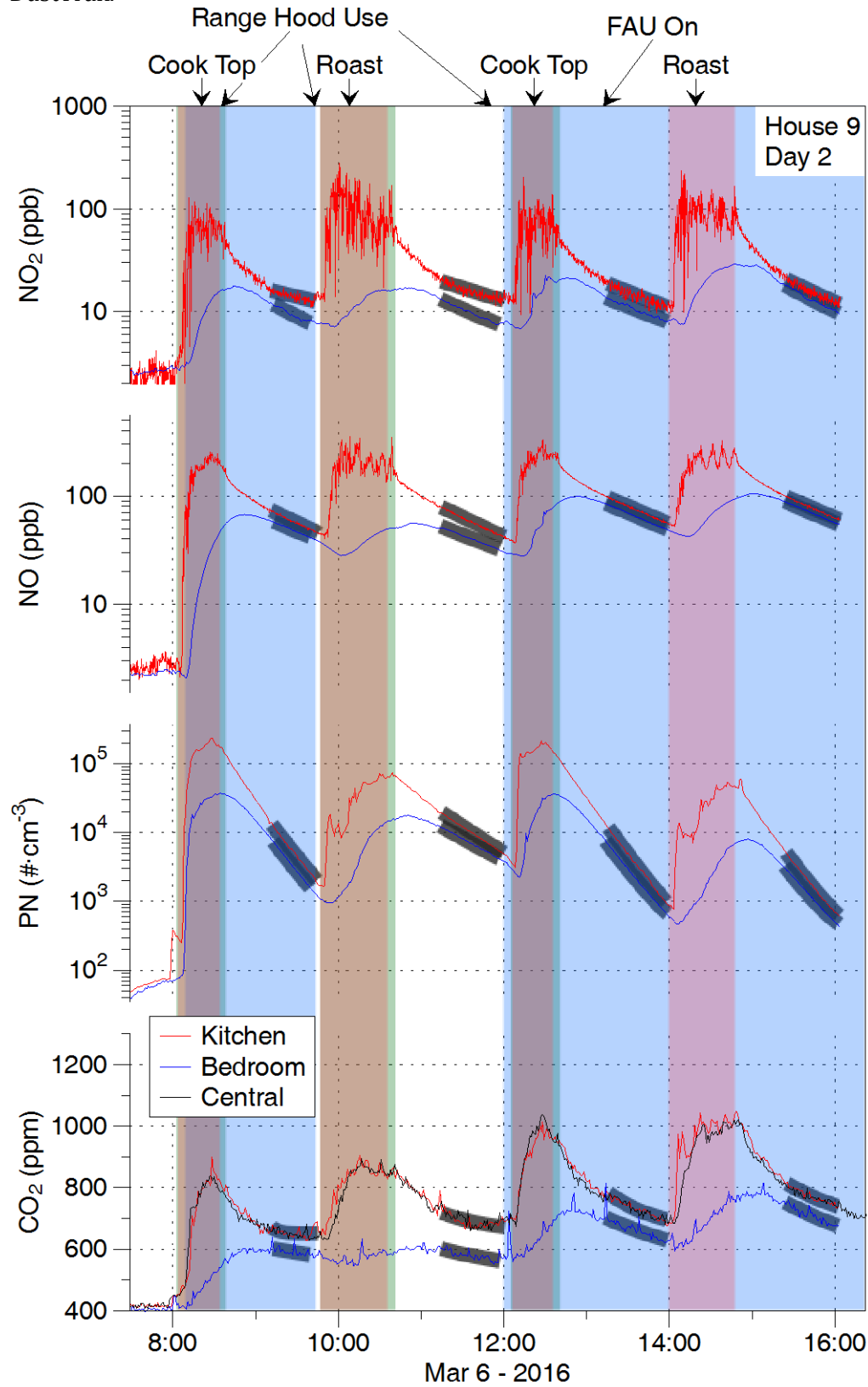
Figure 46. More data from experiments conducted on first day in H09. PM as reported by DustTrak.
