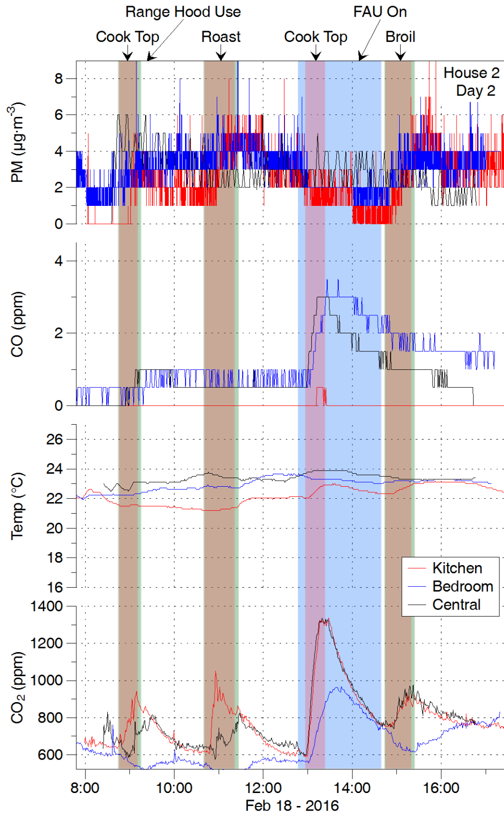
Figure 14. Additional data from experiments conducted on first day in H02. PM as reported by DustTrak.
