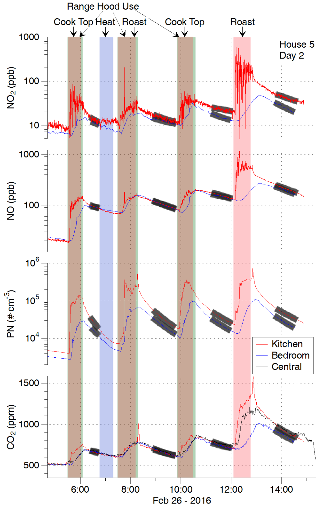
Figure 26. Data from experiments conducted on second day in H05. Grey shading over data interval used to fit decay for disentanglement.
