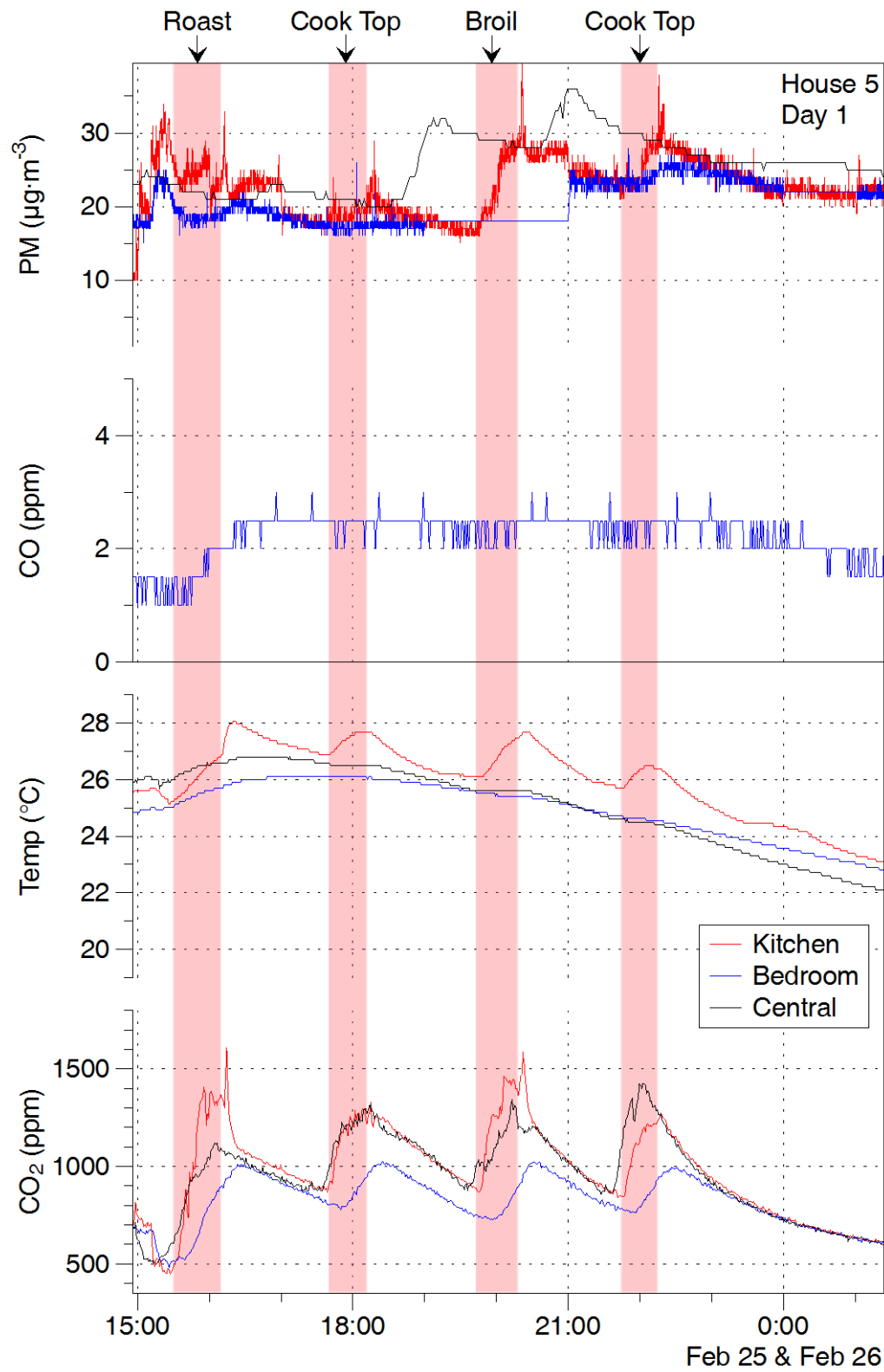
Figure 25. More data from experiments conducted on first day in H05. PM as reported by DustTrak.
