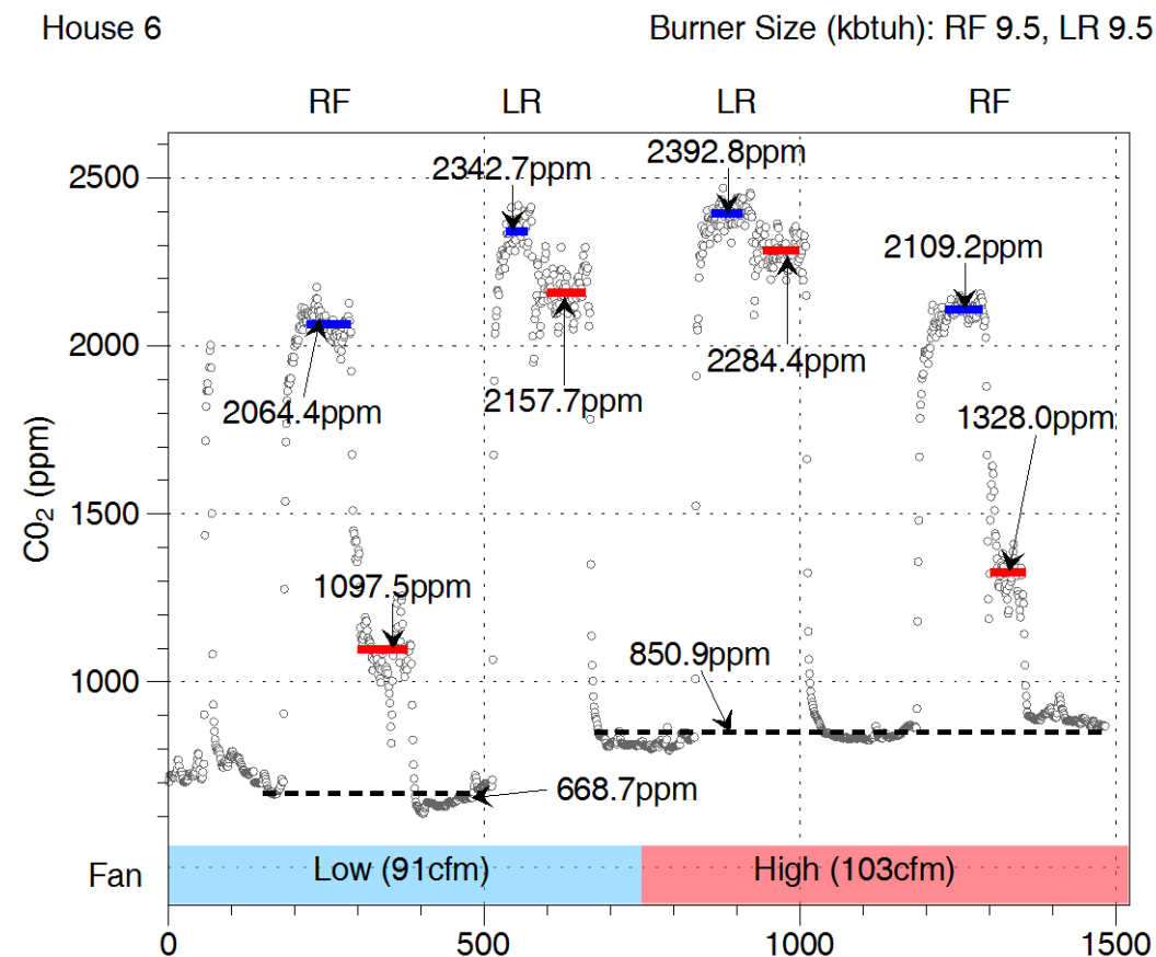
Figure 30. CO 2 data from range hood capture efficiency measurements in H6.
