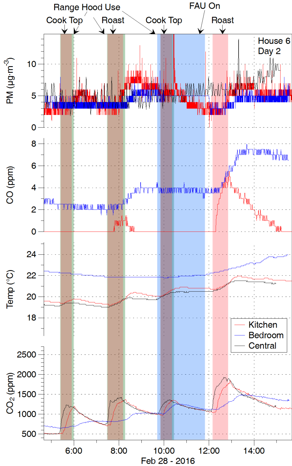
Figure 34. More data from experiments conducted on second day in H6. PM as reported by DustTrak.
