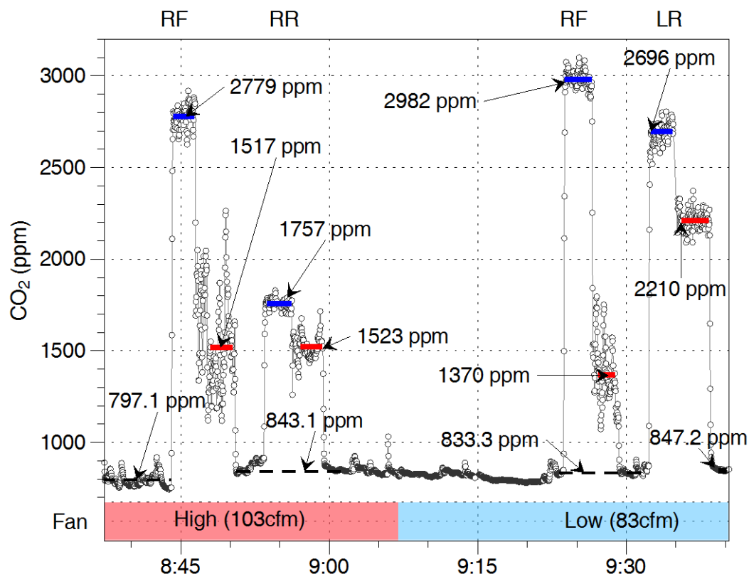
Figure 44. CO 2 data from range hood capture efficiency measurements in H9.
