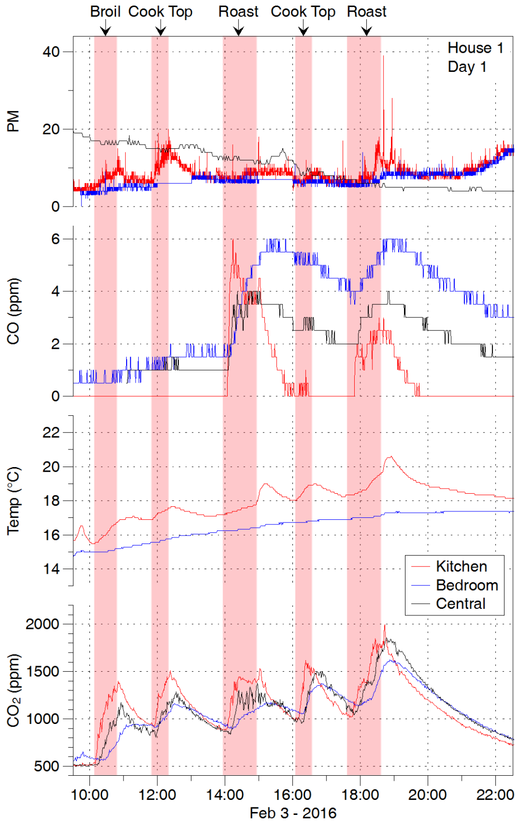
Figure 4. Additional data from experiments conducted on first day in H01. PM as reported by DustTrak.
