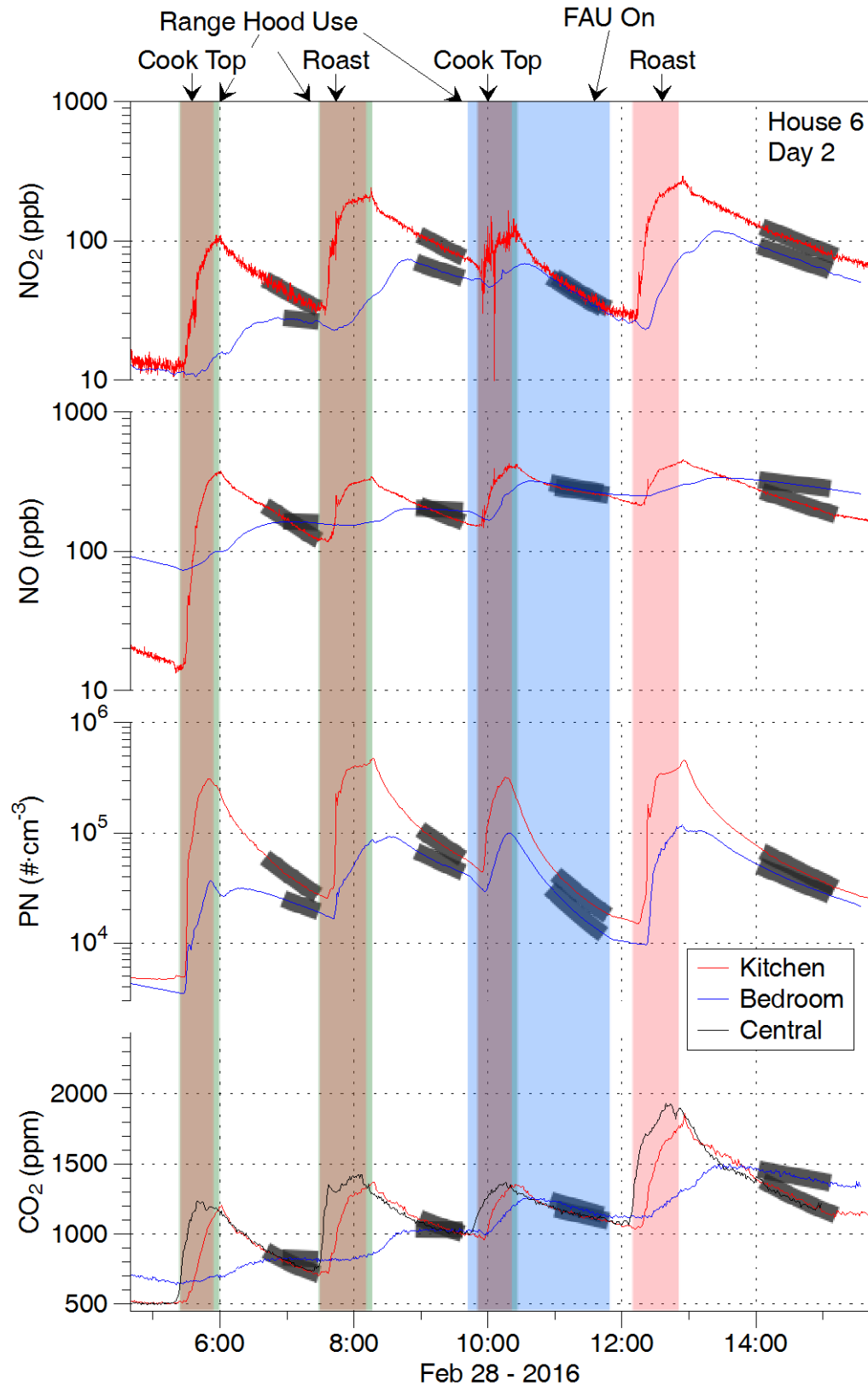
Figure 33. Data from experiments conducted on second day in H6. Grey shading over data interval used to fit decay for disentanglement.
