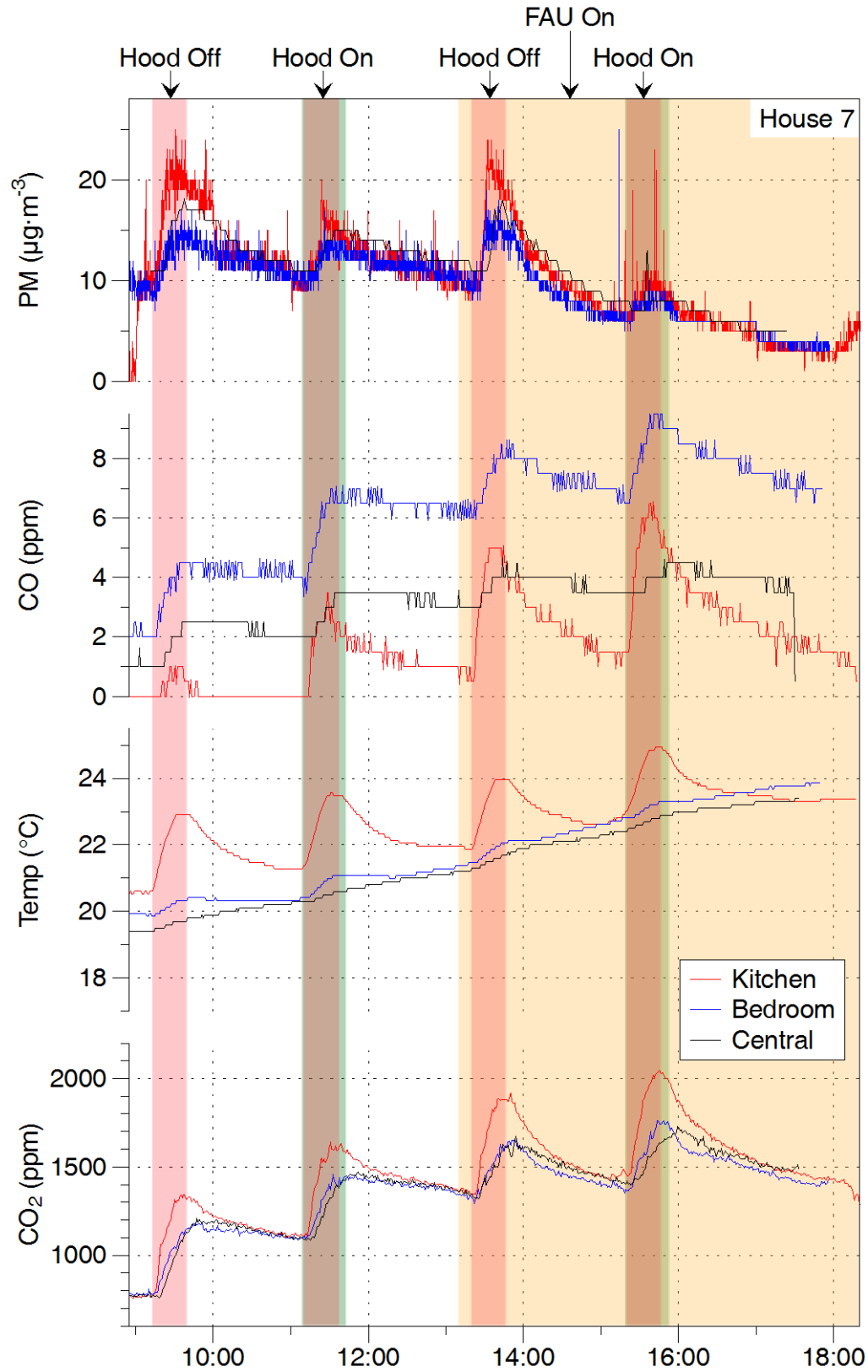
Figure 39. More data from experiments conducted in H07. PM as reported by DustTrak.
