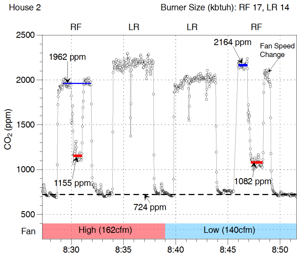
Figure 10. CO 2 data from range hood capture efficiency measurements in H2. The lack of a clear decrease during the measurements for left rear (LR) on high and low speed suggests high capture efficiency for the rear burners.
