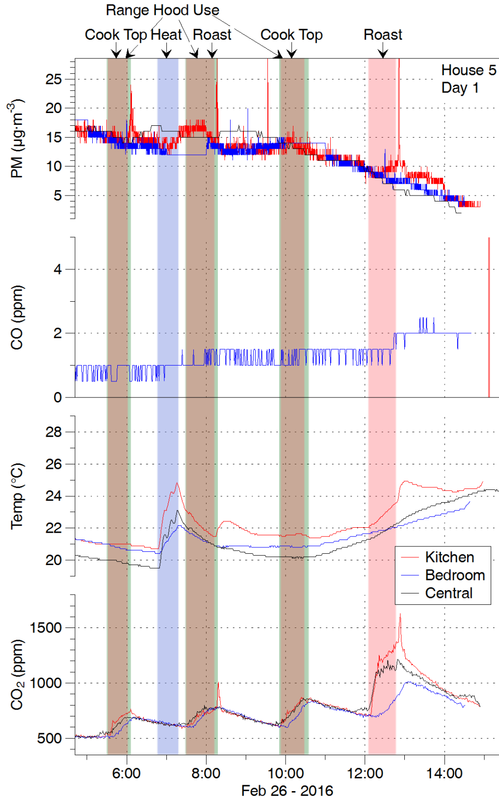
Figure 27. More data from experiments conducted on second day in H05. PM as reported by DustTrak.
