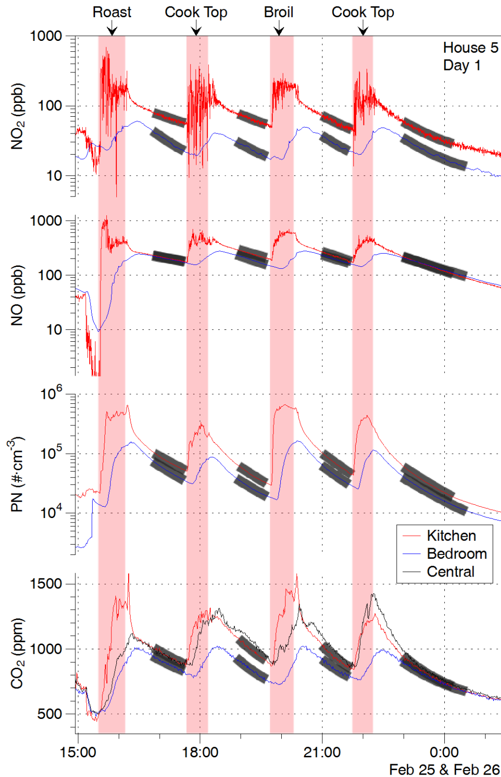
Figure 24. Data from experiments conducted on first day in H05. Grey shading over data interval used to fit decay for disentanglement.
