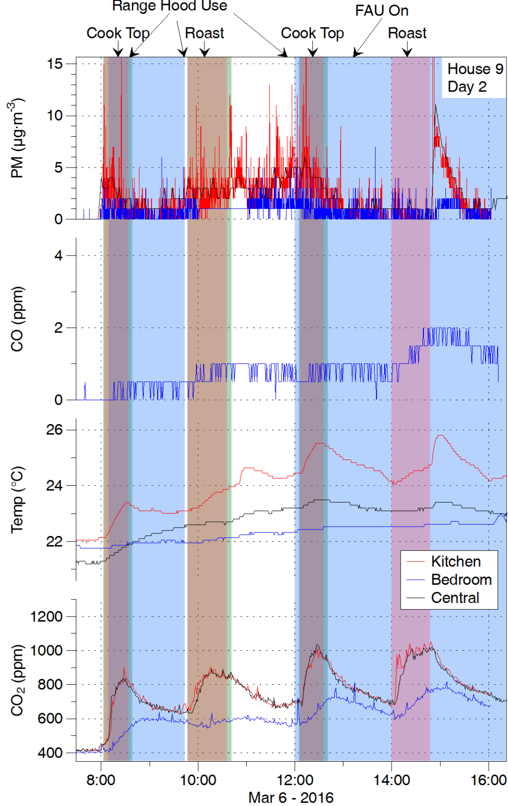
Figure 47. Data from experiments conducted on second day in H9. Grey shading over data interval used to fit decay for disentanglement.
