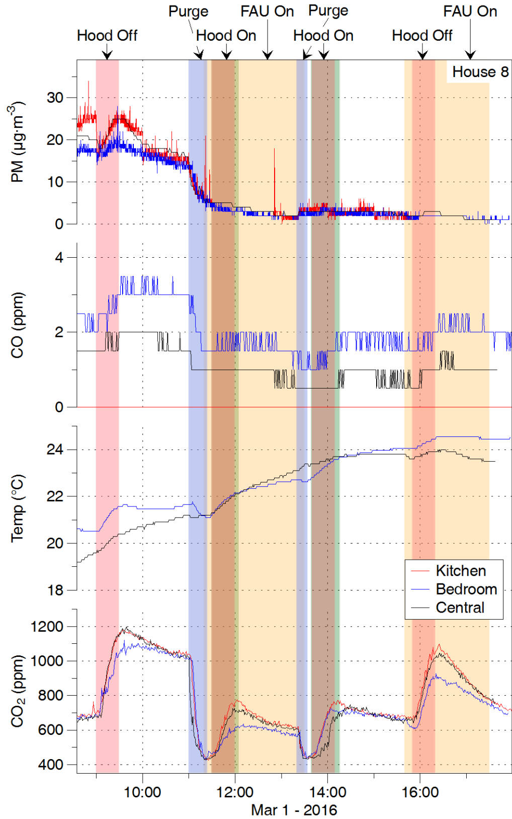
Figure 43. More data from experiments conducted in H08. PM as reported by DustTrak.
