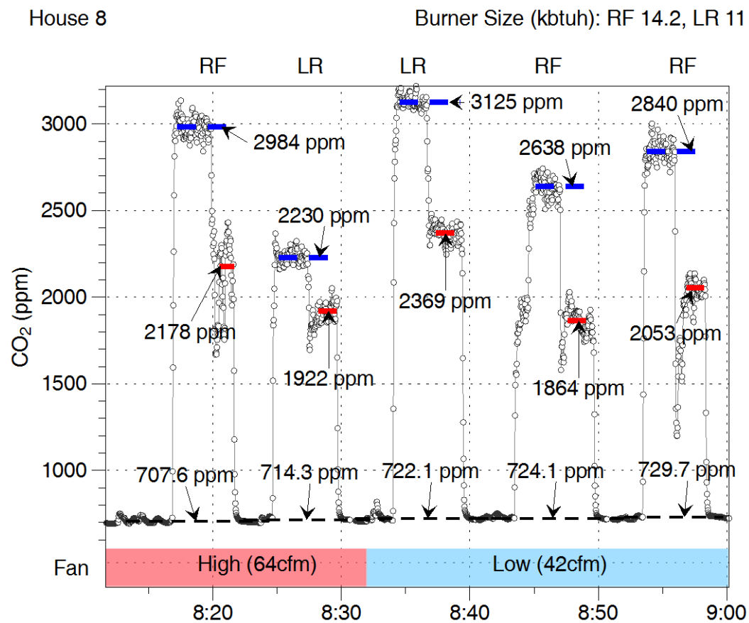
Figure 41. CO 2 data from range hood capture efficiency measurements in H8.
