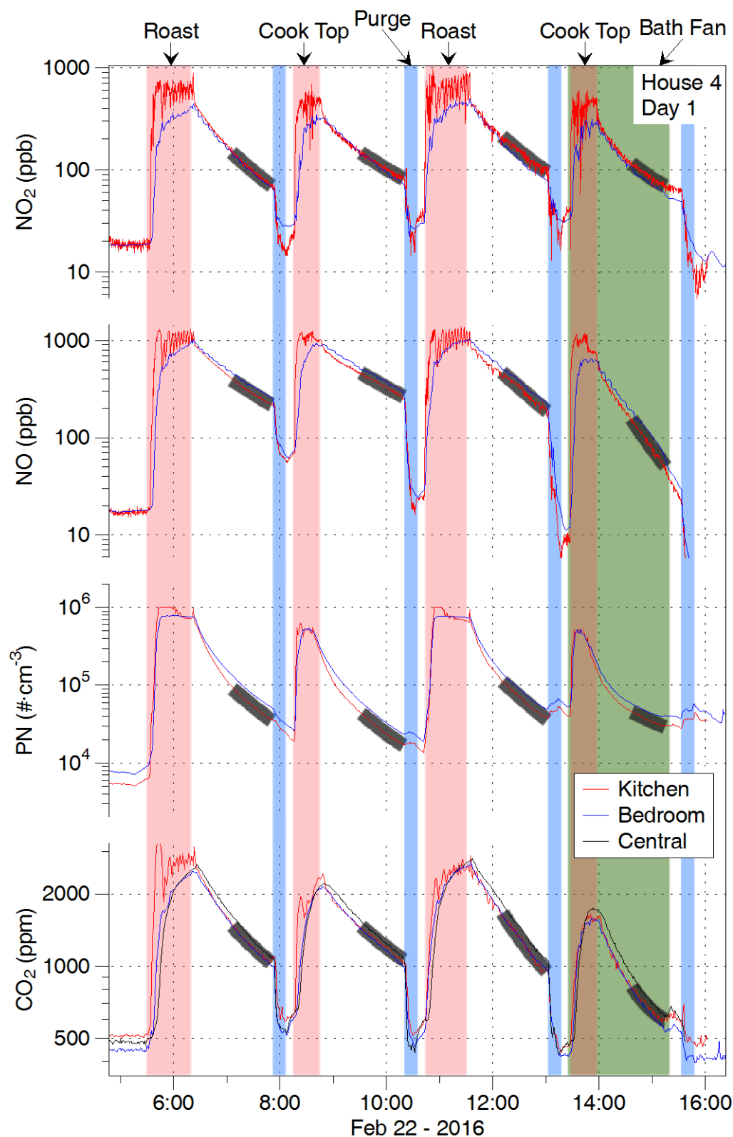
Figure 20. Data from experiments conducted in H4. Grey shading over data interval used to fit decay for disentanglement.
