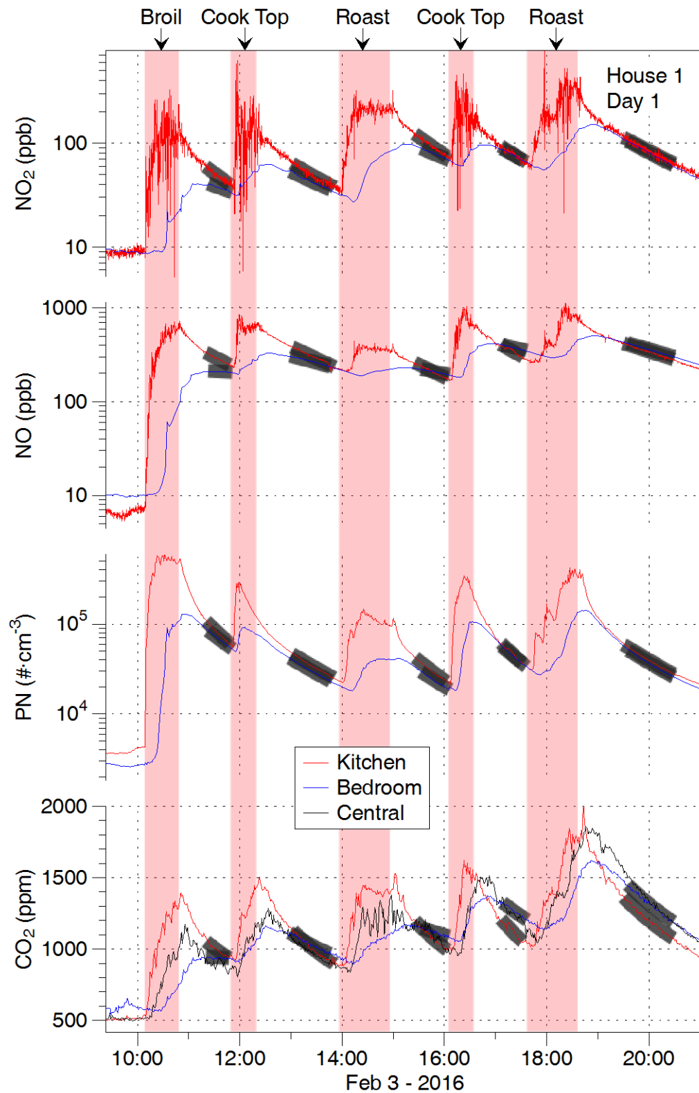
Figure 3. Data from experiments conducted on first day in H01. Grey shading over data interval used to fit decay for disentanglement.
