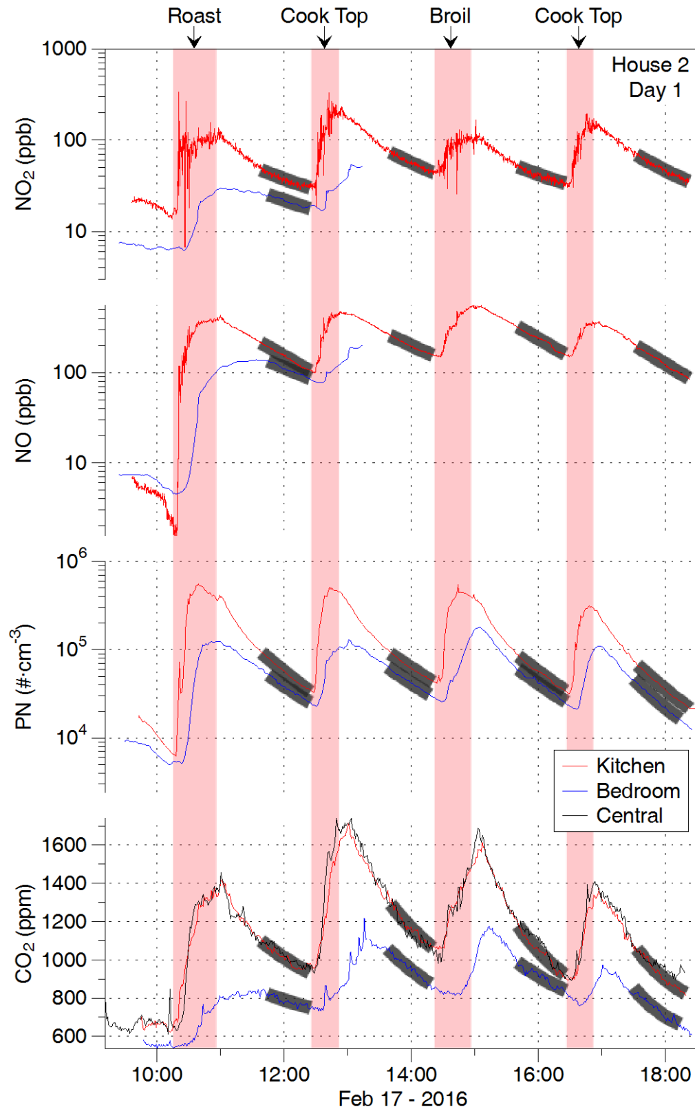
Figure 11. Data from experiments conducted on first day in H2. Grey shading over data interval used to fit decay for disentanglement.
