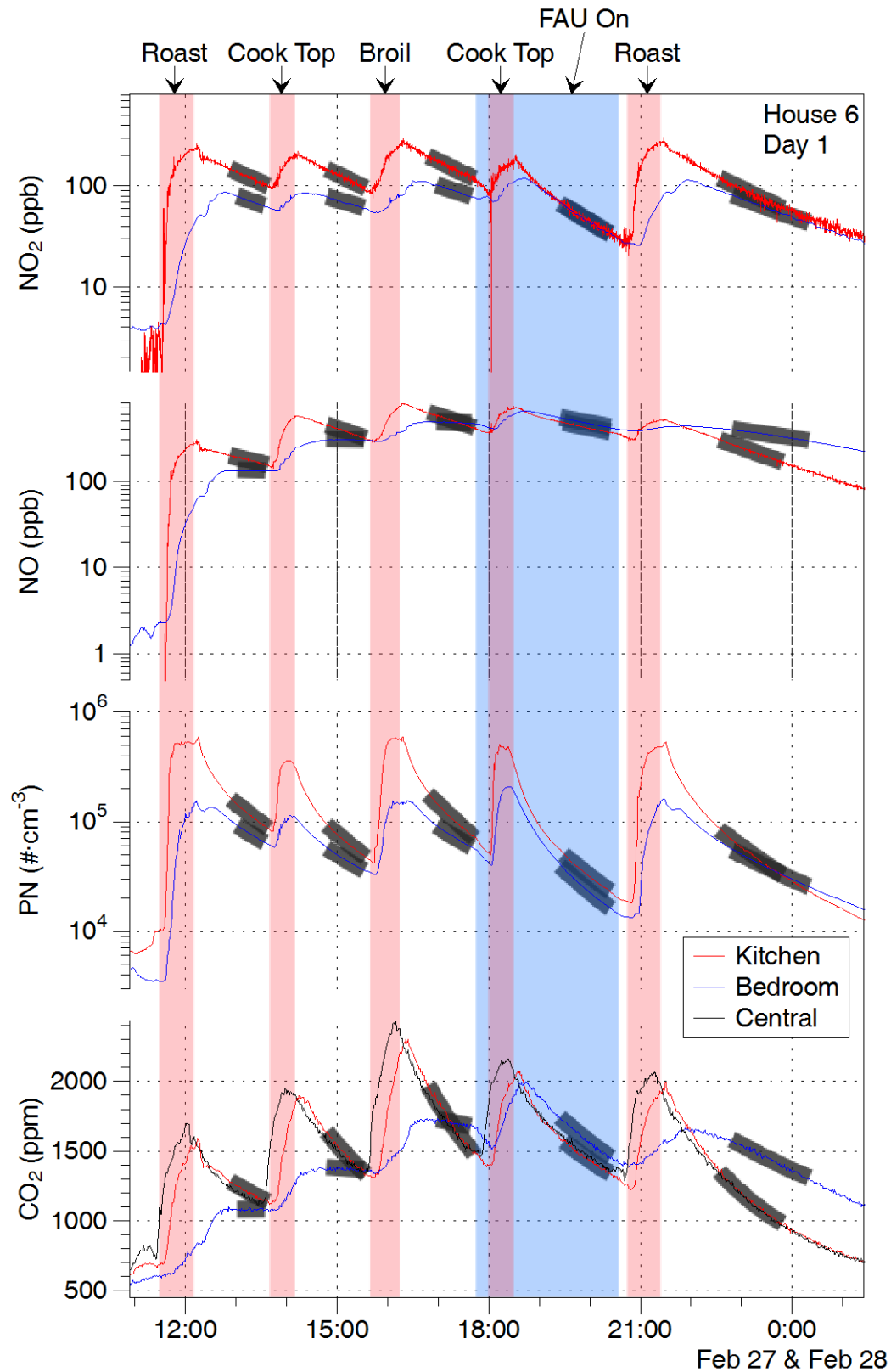
Figure 31. Data from experiments conducted on first day in H06. Grey shading over data interval used to fit decay for disentanglement.
