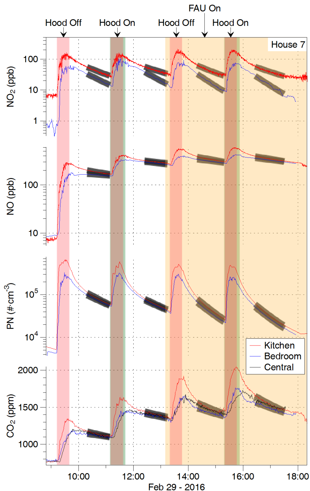
Figure 38. Data from experiments conducted in HO7. Grey shading over data interval used to fit decay for disentanglement.
