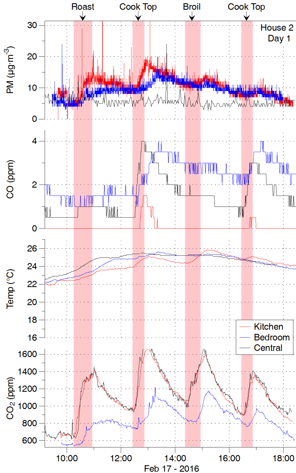
Figure 12. Additional data from experiments conducted on first day in H02. PM as reported by DustTrak.
