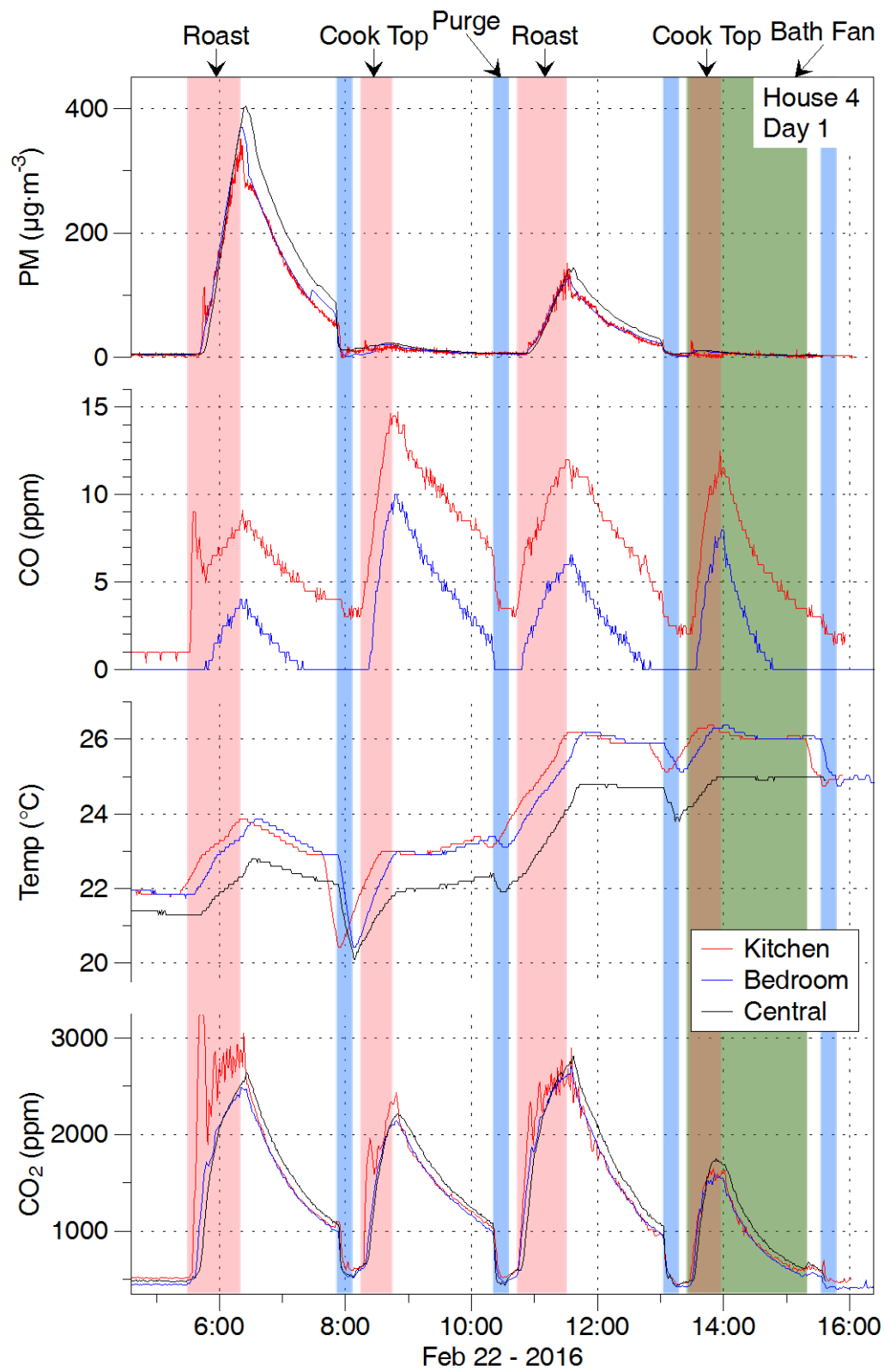
Figure 21. More data from experiments conducted in H4. PM as reported by DustTrak.
