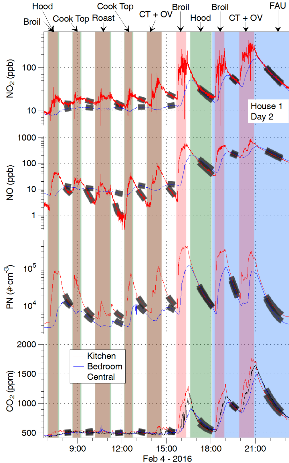
Figure 5. Data from experiments conducted on second day in H01. Grey shading over data interval used to fit decay for disentanglement.
