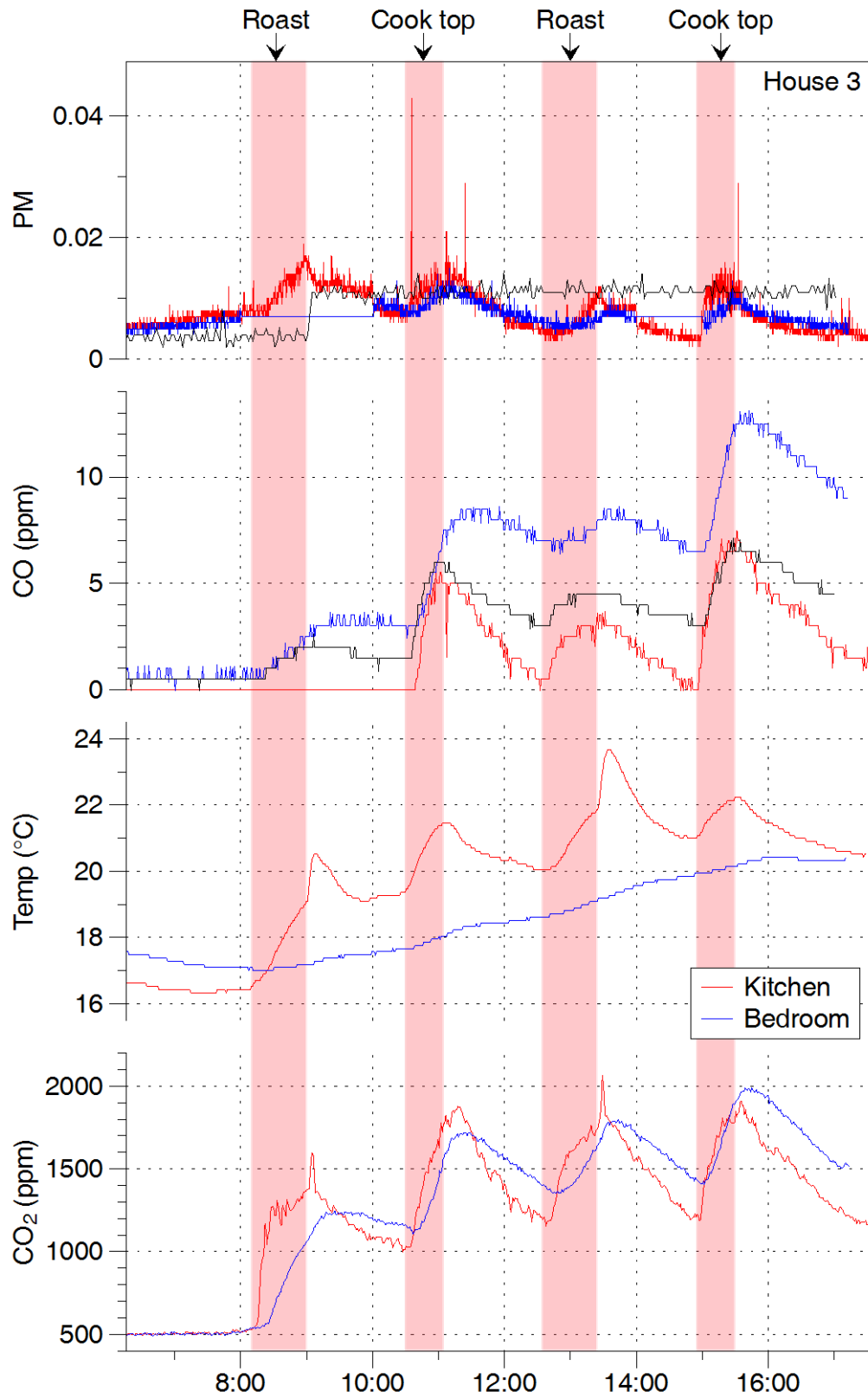
Figure 18. More data from experiments conducted on first day in H03. PM as reported by DustTrak.
