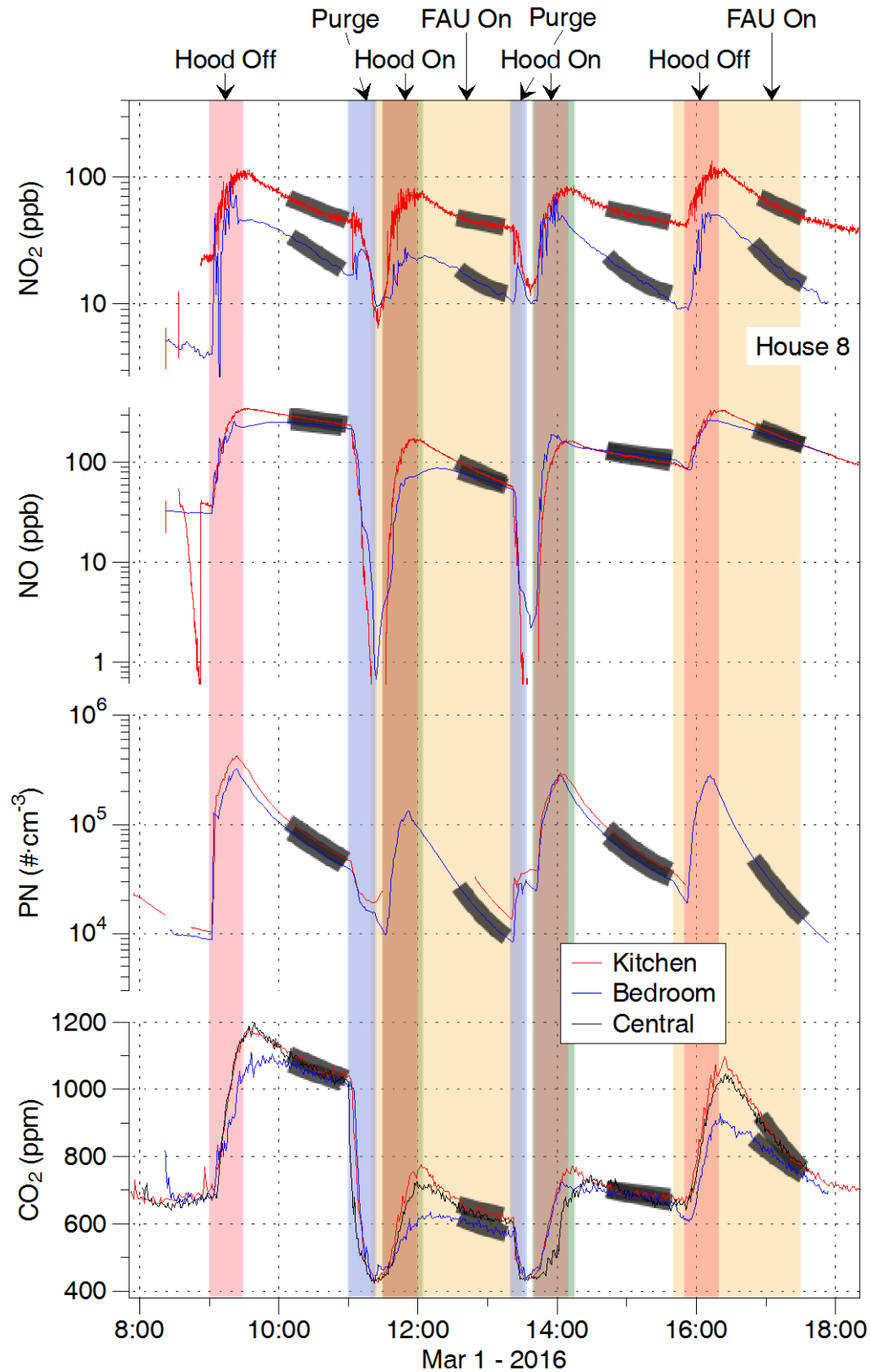
Figure 42. Data from experiments conducted in H08. Grey shading over data interval used to fit decay for disentanglement.
