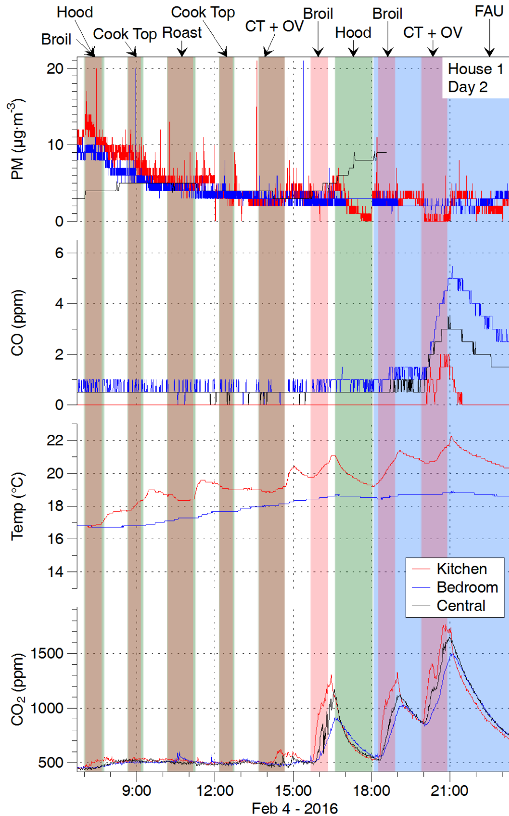
Figure 6. Additional data from experiments conducted on second day in HO1. PM as reported by DustTrak.
