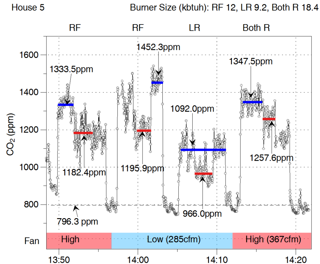
Figure 23. CO 2 data from range hood capture efficiency measurements in H5.
