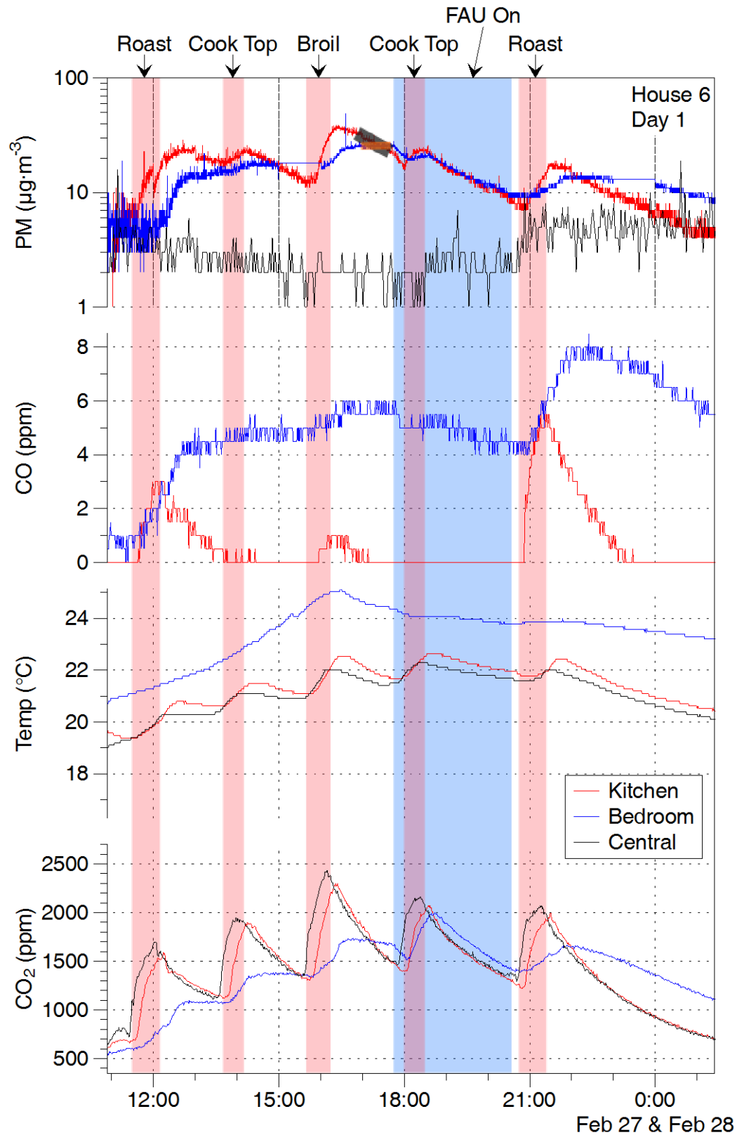
Figure 32. More data from experiments conducted on first day in H06. PM as reported by DustTrak.
