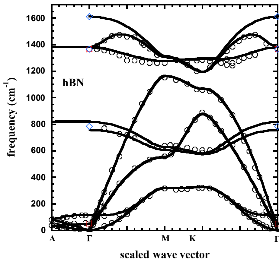
Figure S3: Calculated phonon dispersion of bulk hBN (black curves) compared with measured data from Raman (red squares) 16 , IR (blue diamonds) 17 and x-ray (black open circles) 18 experiments.
