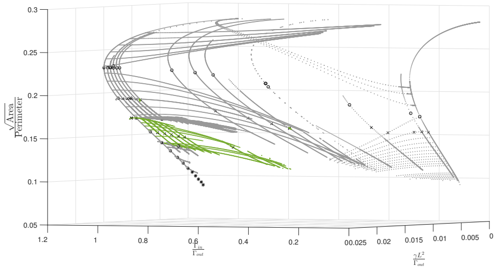
Figure 4.14: The family of Sadvskii solutions connecting the doubly cusped solutions at the m = 4 patch bifurcation with the solutions with two pinch off points at the m = 6 patch bifurcation is shown in green. All other Sadvskii solutions are shown in grey.
