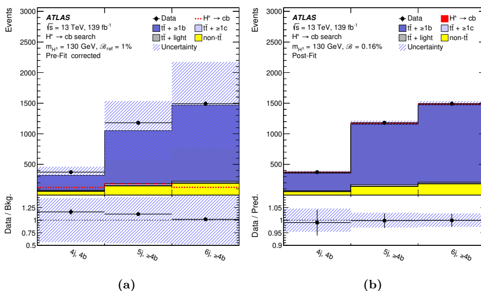
Figure 7. Comparison between the data and prediction for the event yields in the fit regions (4j, 4b), (5j, \geq 4b ) and (6j, \geq 4b ) (a) before the likelihood fit to data (“Pre-Fit”), and (b) after the likelihood fit to data (“Post-Fit”). The small contributions from t\bar{t}V , t\bar{t}H , single-top-quark, W/Z +jets, diboson, tHq and tZq backgrounds are combined into a single background source referred to as “non- t\bar{t} ”. The pre-fit H^\pm signal for m_{H^\pm} = 130 GeV is displayed as a dashed red line normalised to \mathcal{B}_{\text{ref}} = 1\% . The post-fit H^\pm signal for m_{H^\pm} = 130 GeV is displayed as a red histogram normalised to the best-fit branching fraction of 0.16%, added on top of the background prediction. The bottom panels display the ratios of data to either the SM background prediction before the fit (“Bkg”) or the total signal-plus-background prediction after the fit (“Pred”). The hashed area represents the total uncertainty of the background. The t\bar{t} background prediction is corrected according to the procedure described in section 5.2.
