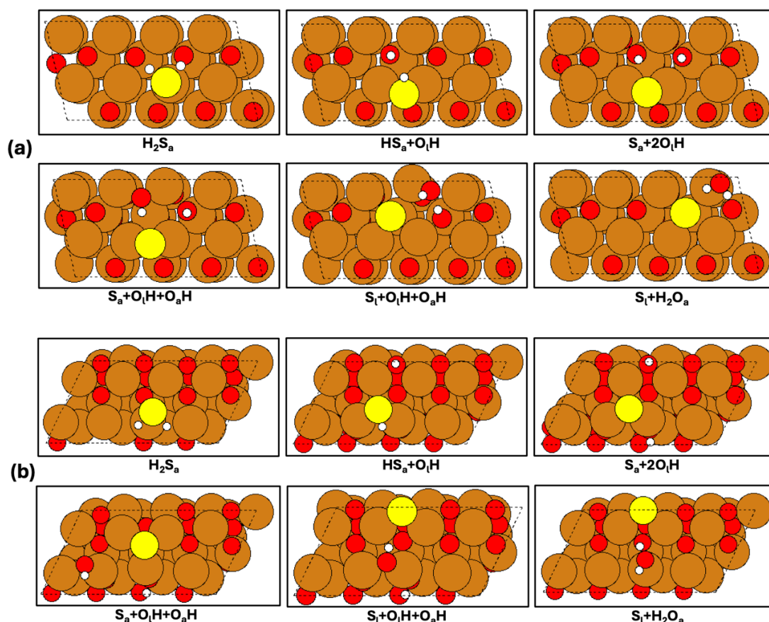
Figure 3. Structures for reaction intermediates involving a) O_{3c} with a single H_2S molecule on bare CuO (111) surface b) and O_{3c} with a single H_2S molecule on bare CuO ( \bar{1}\bar{1}\bar{1} ) surface. Oxygen atoms are shown in red and copper atoms in brown and sulfur atoms in yellow.
