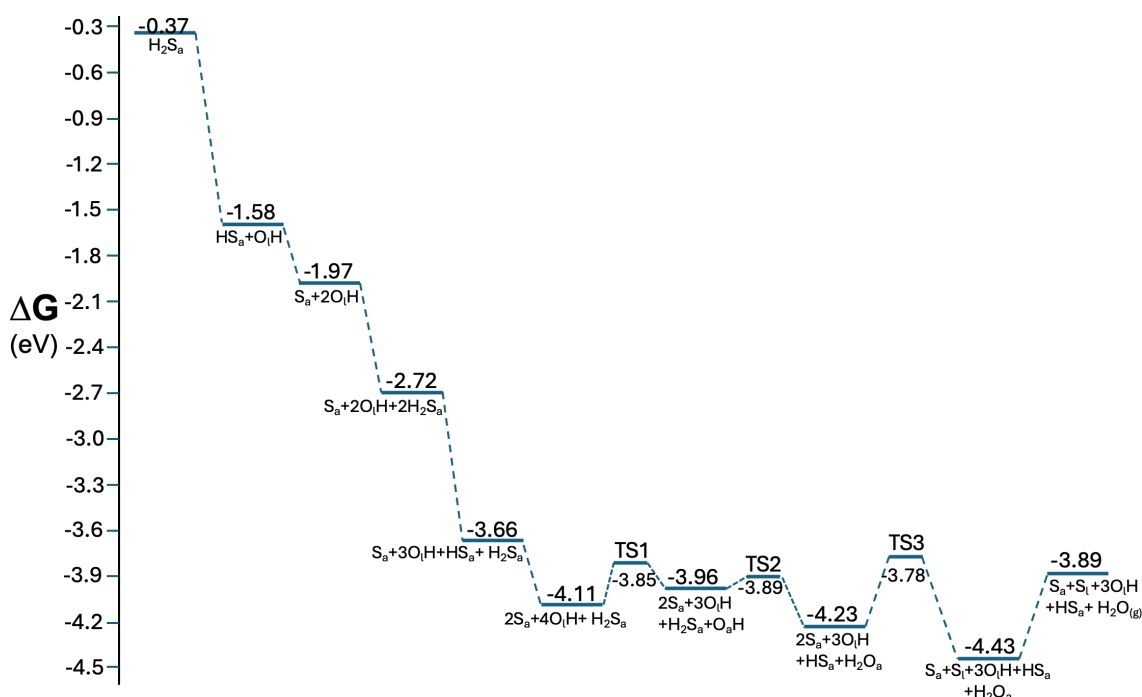
Figure 6. Reaction profile showing the change in Gibbs free energy versus elementary reaction steps for reaction of three \text{H}_2\text{S} molecules on the \text{CuO} ( \bar{1}11 ) surface. After the second deprotonation of the first \text{H}_2\text{S} molecule ( \text{S}_a+2\text{O}_i\text{H} ), a second and third \text{H}_2\text{S} are added simultaneously and reacted until the formation of a single \text{H}_2\text{O} molecule. Corresponding structures are shown in Figure 7. For the free energy calculation, T = 298 \text{ K} and P = 101 \text{ Pa} .
