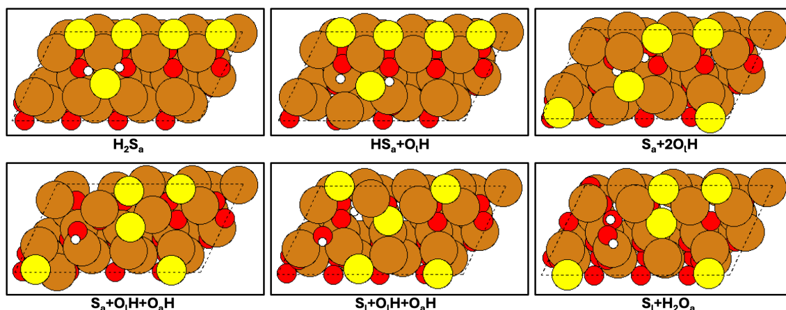
Figure 11. Stable structures along the reaction pathway of Figure 10 for reaction of O_{4c} on the partially sulfided CuO ( \bar{1}\bar{1}\bar{1} ) surface.
