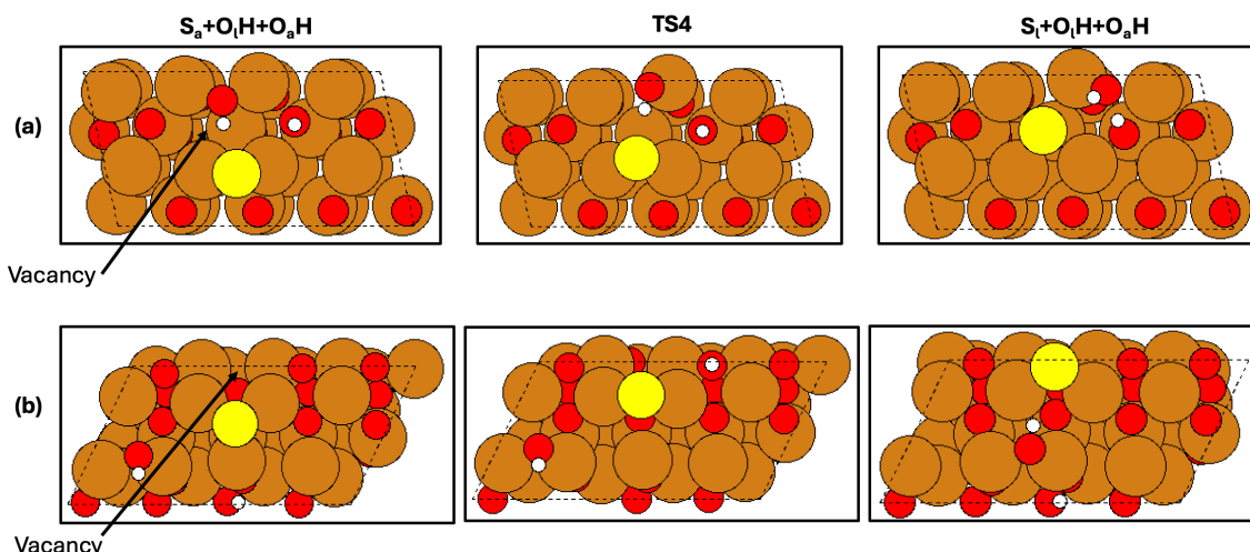
Figure 4. Structures of transition states (TS4 in Figure 2) and corresponding initial and final elementary step structures for the healing of the oxygen vacancy by the surface S atom, comparing O_{3c} pathways on a) the CuO (111) surface and on b) the CuO ( \bar{1}\bar{1}1 ) surface. A change in the hydroxyl coordination to Cu is required on the CuO (111) surface to expose the vacancy to S.
