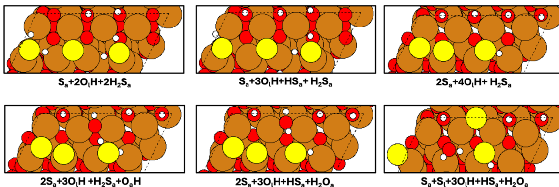
Figure 7. Stable structures along the reaction pathway of Figure 6 involving the addition of a second and third \text{H}_2\text{S} to the \text{O}_{3c} ( \bar{1}11 ) pathway after the second deprotonation of the first \text{H}_2\text{S} and reaction until the formation of a single \text{H}_2\text{O} molecule.
