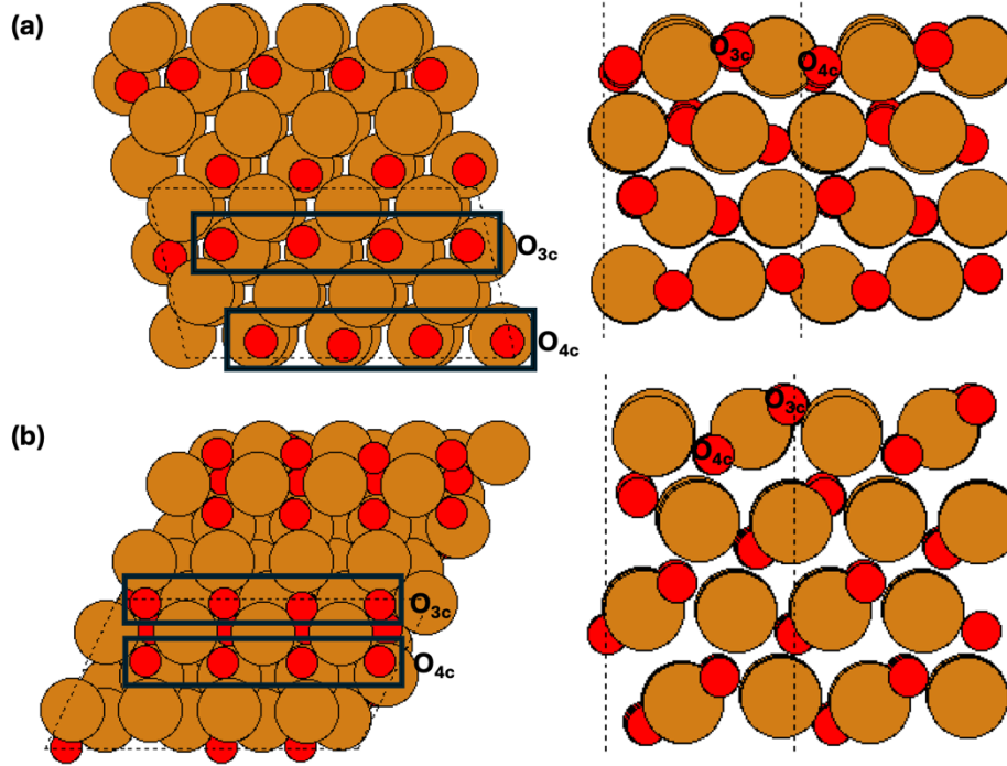
Figure 1. Top (left) and side (right) view of the surface models for the a) CuO (111) surface b) CuO ( \bar{1}\bar{1}1 ) surface considered in this study. Oxygen atoms are shown in red and copper atoms shown in brown. Dashed lines indicate unit cell boundaries. Black boxes indicate rows of three coordinated and four coordinated oxygens.
