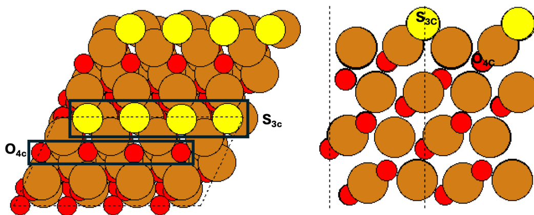
Figure 9. Top and side view of surface models for partially sulfided CuO ( \bar{1}11 ) surface. Each S_{3c} is a three-coordinated sulfur atom occupying the lattice sites initially occupied by a O_{3c} surface atom.
