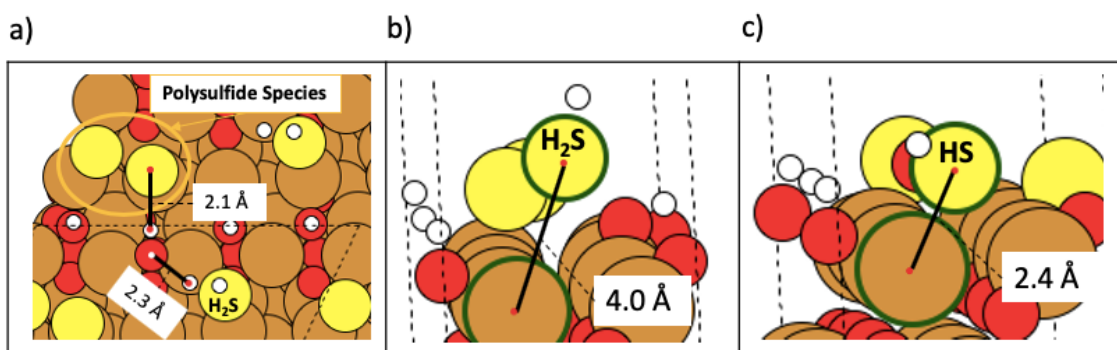
Figure 8. Structures of a) OH migration top view showing stabilizing interactions b) OH migration side view showing \text{H}_2\text{S} physisorption and c) water formation showing HS chemisorption on the surface for the reaction involving addition of 2 \text{H}_2\text{S} to the \text{O}_{3c} ( \bar{1}11 ) pathway.
