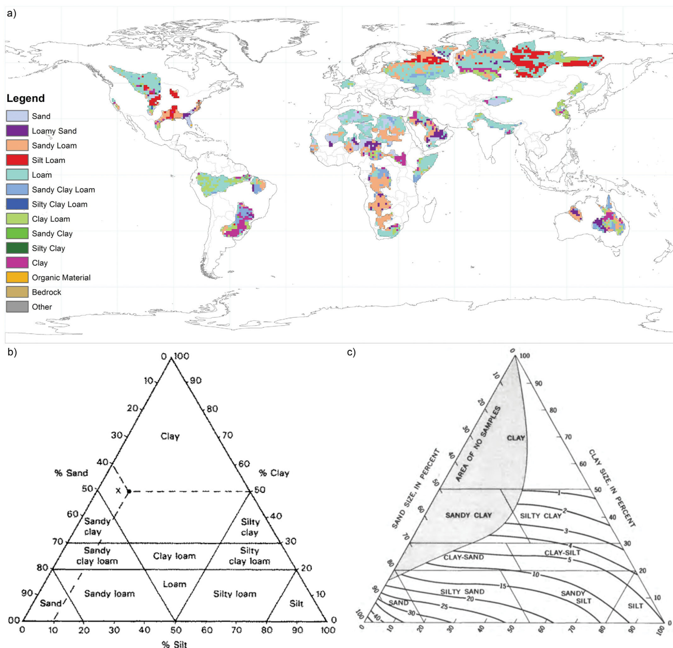
Figure 2. (a) 1^\circ \times 1^\circ global-gridded USDA soil texture class map in the study aquifers derived for GLDAS [Rodell et al., 2004a] based on percentages of sand, silt, clay from the soils data set of Reynolds et al. [2000] used to determine the dominant soil type in each aquifer system. (b) Simplified soil classification triangle based on percentages of sand, silt, and clay [ILO, 1987]. (c) Soil classification triangle coupled with estimates of specific yield from Johnson [1967] to determine the range of specific yields associated with each soil type. The contours represent specific yield as a percentage.
