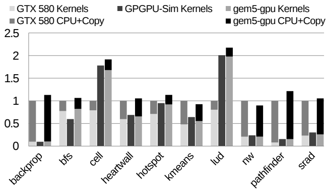
Fig. 2. Run times normalized to NVIDIA GTX 580.
