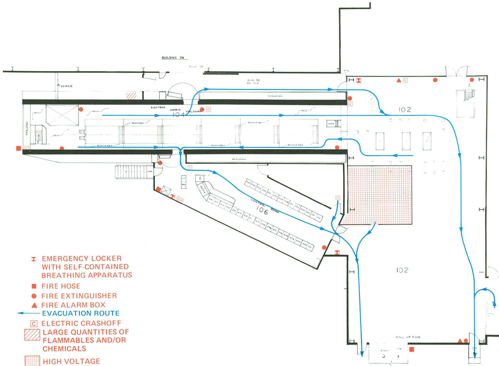
Fig. 6. Building 58A, FIRST FLOOR, evacuation routes, fire equipment, and hazard areas.
