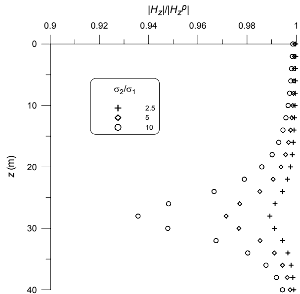
Figure 7. Sensitivity in the amplitude of the vertical magnetic field along a vertical profile 40 m from the transmitter. The anomaly is caused by a conductor 5 m thick and 20 m wide in radius with varying conductivity, in a background of 0.01 S/m.
