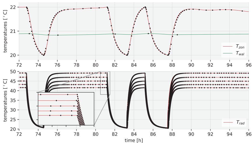
Figure 8: Trajectories computed by CVode (red) and points (black) at which QSS updates the respective state for the model in Figure 7. For easier readability, for QSS only every 5th state update is drawn.
