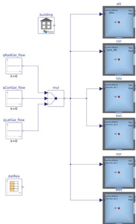
Figure 3: Modelica model of the office building used to validate the EnergyPlus-Modelica coupling.
