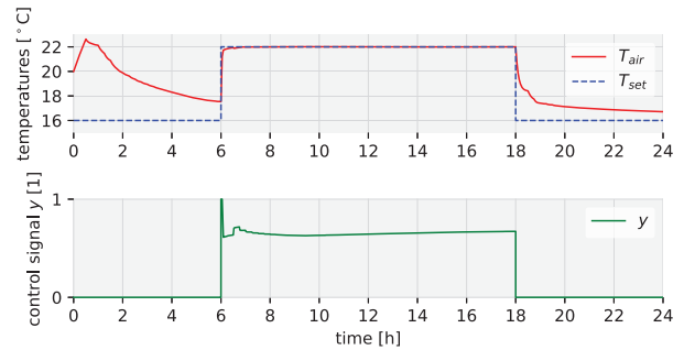
Figure 6: Room air temperature T_{air} , room air temperature set point T_{set} and resulting control signal y for the model in Figure 5.
