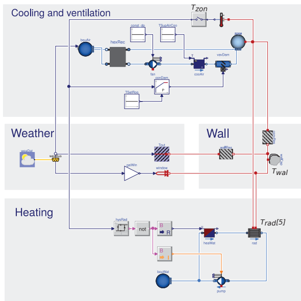
Figure 7: Modelica model used for the QSS example.
