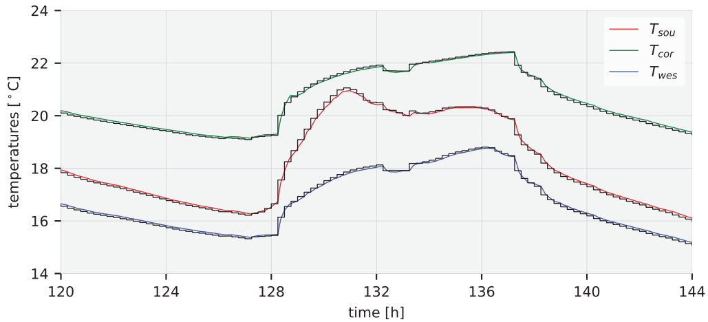
Figure 4: Free floating room air temperatures for south, core and west zones for the DOE small office reference building for Chicago, IL, shown in Figure 3. Black lines are from legacy EnergyPlus, and colored lines are from Spawn.
