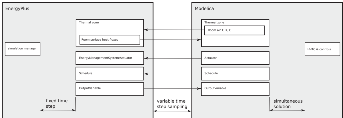
Figure 2: Partitioning of the envelope, room and HVAC model.
