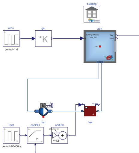
Figure 5: Coupling a simple Modelica HVAC system model to an EnergyPlus envelope model.
