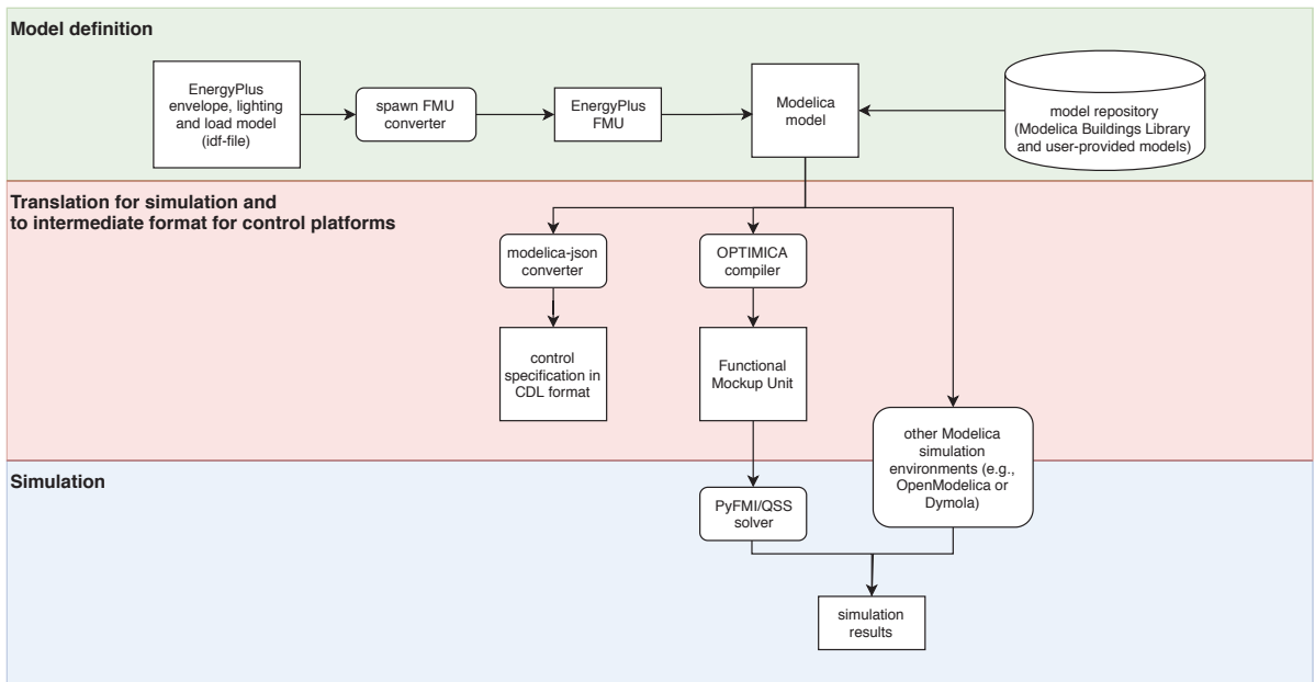
Figure 1: Architectural diagram of Spawn.
