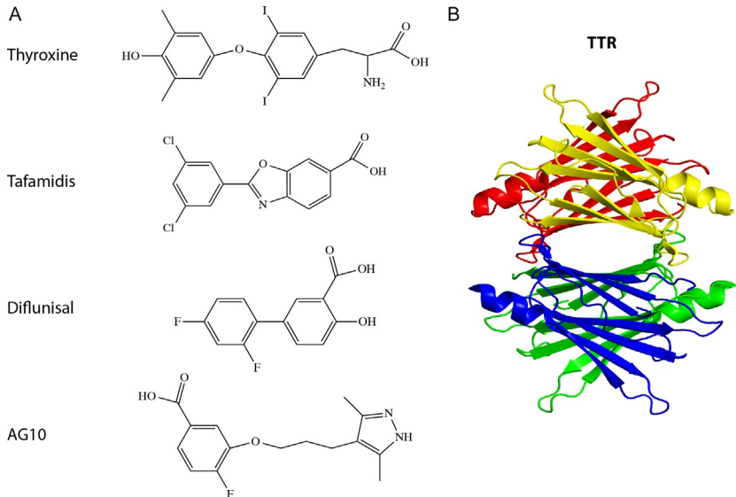
Fig. 1 TTR and its ligands. (A) Schematic structures of the thyroid hormone, thyroxine, a natural ligand of TTR, and of the TTR ligands tafamidis, an FDA-approved drug for FAP, diflunisal, available off-label for TTR amyloidoses, and AG10, a compound in clinical trial for FAC. (B) A ribbon diagram of TTR showing the tetramer structure composed of yellow, red, blue, and green monomers.
