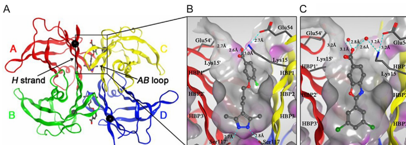
Fig. 2 Crystal structures of V122I-TTR ligand complexes. (A) Quaternary structure of AG10 bound to V122I-TTR shown as a ribbon representation with monomers colored individually and positions of each of the V122I mutations shown as black spheres located on the H\beta -strand, which interacts with the adjacent AB -loop on the AC/BD interface. (B) AG10 in complex with V122I-TTR. (C) Tafamidis in complex with V122I-TTR. Close-up views of one of the two identical thyroxine binding sites with different colored ribbons for the two monomers of the tetramer composing the binding site. A Connolly molecular surface 15 was applied to residues within 10 Å of ligand in the thyroxine binding pocket and colored gray for hydrophobic and purple for polar residues. Reproduced from reference Penchala SC, Connelly S, Wang Y, Park MS, Zhao L, Baranczak A, et al. AG10 inhibits amyloidogenesis and cellular toxicity of the familial amyloid cardiomyopathy-associated V122I transthyretin. Proc. Natl. Acad. Sci. USA 2013;110:9992–9997.
