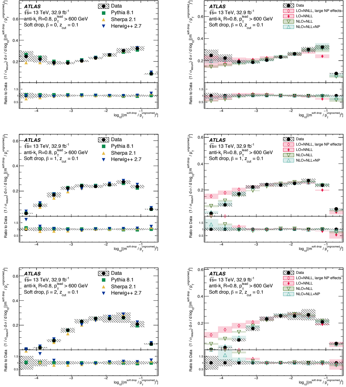
Figure 3: The unfolded \log_{10}(\rho^2) distribution for anti- k , R = 0.8 jets with p_T^{\text{lead}} > 600 GeV, after the soft drop algorithm is applied for \beta \in \{0, 1, 2\} , in data compared to PYTHIA, SHERPA, and HERWIG++ particle-level (left), and NLO+NLL(+NP) [15] and LO+NNLL [17, 18] theory predictions (right). The LO+NNLL calculation does not have non-perturbative (NP) corrections; the region where these are expected to be large is shown in an open marker (but no correction is applied), while regions where they are expected to be small are shown with a filled marker. All uncertainties described in the text are shown on the data; the uncertainties from the calculations are shown on each one. The distributions are normalized to the integrated cross section, \sigma_{\text{resum}} , measured in the resummation region, -3.7 < \log_{10}(\rho^2) < -1.7 . The NLO+NLL+NP cross-section in this resummation regime is 0.14, 0.19, and 0.21 nb for \beta = 0, 1, 2 , respectively [15].
