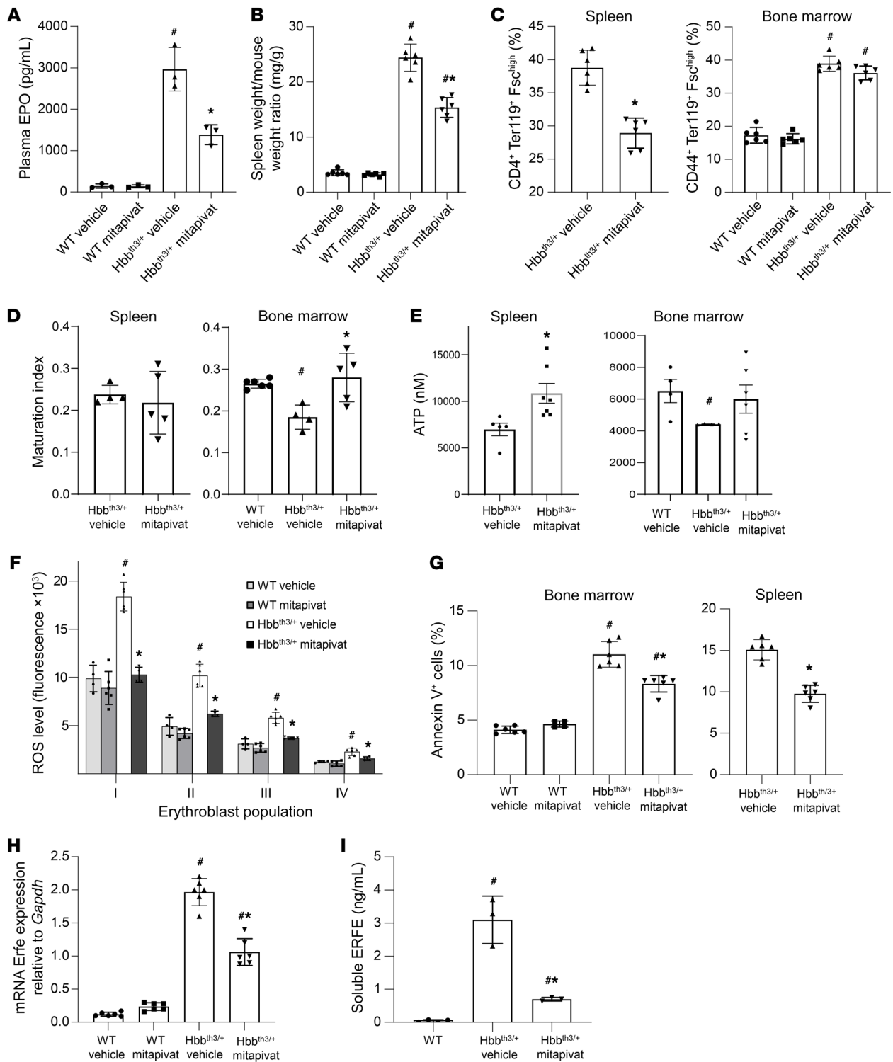
Figure 2. Mitapivat ameliorated ineffective erythropoiesis in Hbb th3/+ mice. (A) Plasma EPO in WT and Hbb th3/+ mice. Data are mean ± SD (n = 3). (B) Spleen weight/mouse weight ratio in WT and Hbb th3/+ mice. Mean ± SD (n = 6). (C) Flow cytometry (CD44-Ter119 and cell size markers) of bone marrow and spleen from WT and Hbb th3/+ mice. Mean ± SD (n = 6). (D) Ratio of proerythroblasts plus basophilic erythroblasts/polychromatic plus orthochromatic erythroblasts (maturation index) in spleen and bone marrow from Hbb th3/+ mice by flow cytometry. Mean ± SD ( Hbb th3/+ , n = 4 vehicle-treated, n = 5 mitapivat-treated; WT, n = 6). (E) ATP content in sorted CD44-Ter119 total erythroblasts from spleen and bone marrow of Hbb th3/+ mice and bone marrow of WT mice. Mean ± SEM (spleen, vehicle-treated, n = 5, versus mitapivat-treated, n = 7; P < 0.05; bone marrow, WT vehicle, n = 4, Hbb th3/+ vehicle-treated, n = 4, versus mitapivat-treated, n = 6; P = NS). (F) ROS levels in erythroblasts from WT or Hbb th3/+ mice. Mean ± SD (WT, n = 4 vehicle-treated and n = 6 mitapivat-treated; Hbb th3/+ , n = 6 vehicle and n = 4 mitapivat-treated). (G) Annexin-V + erythroid cells from WT or Hbb th3/+ mice. Mean ± SD (WT, vehicle-treated n = 6 and mitapivat-treated n = 4; Hbb th3/+ , n = 6 each group). (H) mRNA expression of Erfc by qRT-PCR of sorted erythroblasts from bone marrow of WT and Hbb th3/+ mice. Mean ± SD, n = 6. (I) Soluble plasma ERFE levels in WT and Hbb th3/+ . Mean ± SD (WT, vehicle-treated n = 4; Hbb th3/+ , n = 3 each group). (A–D, F–I) #P < 0.05 versus WT mice and *P < 0.05 versus vehicle-treated mice by 2-way ANOVA with Bonferroni multiple comparison correction.
