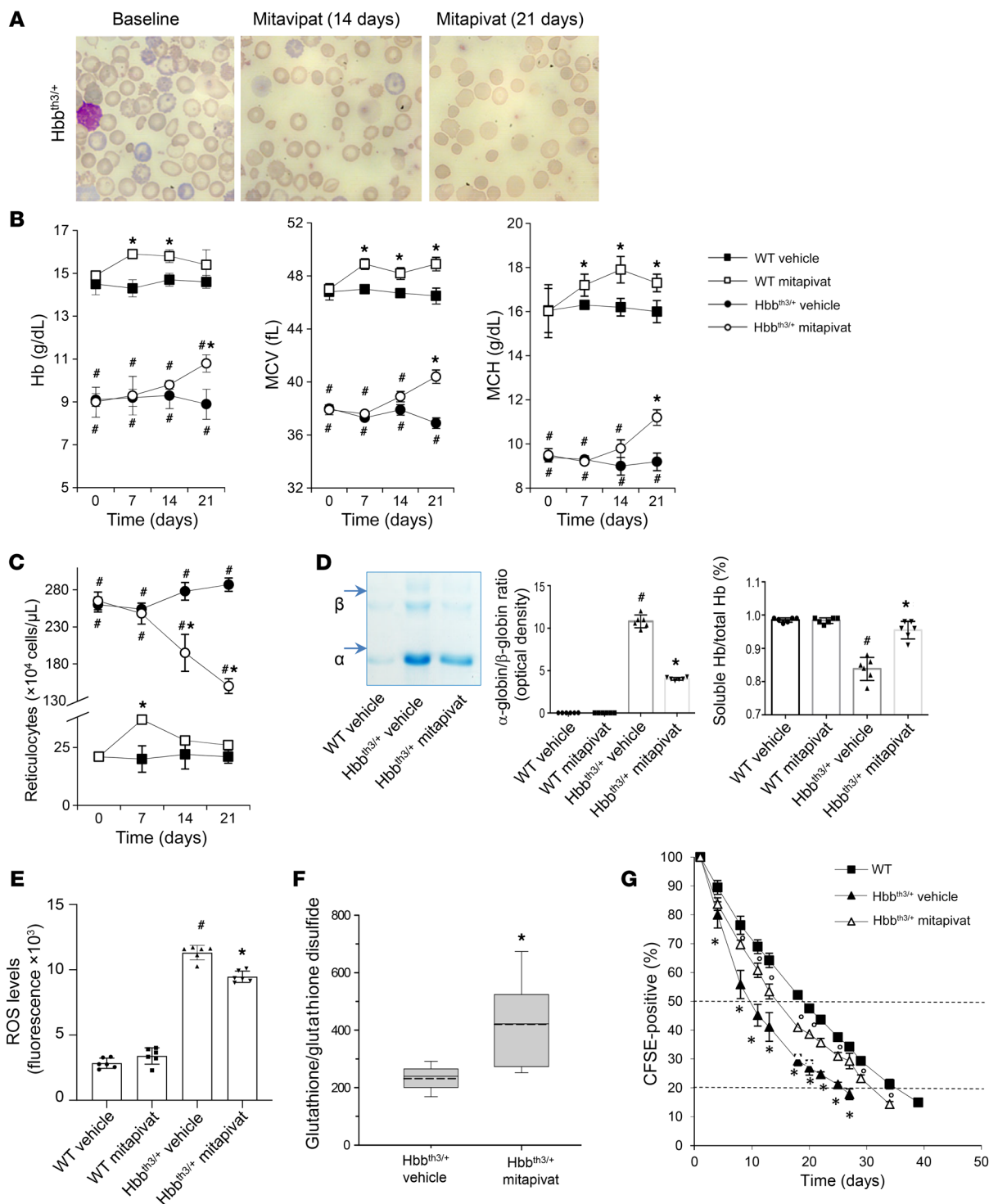
Figure 1. Mitapivat treatment improved chronic hemolytic anemia and red cell survival in the Hbb th3/+ mouse model of \beta -thalassemia. WT and Hbb th3/+ mice were treated with vehicle or mitapivat 50 mg/kg twice daily. (A) Erythrocyte morphology. One representative image from 8 with similar results shown. Original magnification \times 100 . (B and C) Hb, MCV, MCH, and reticulocyte count in WT and Hbb th3/+ mice treated with vehicle or mitapivat. Data are mean \pm SD ( n = 6 ). (D, left panel) Triton acid-urea gel electrophoresis of red cell membrane from WT and Hbb th3/+ mice treated with vehicle or mitapivat (21 days). Arrows show \alpha -globin and \beta -globin associated with red cell membrane. (D, middle panel) Gel quantification expressed as \alpha -globin/ \beta -globin ratio to Hb. Data are mean \pm SD ( n = 6 ). (D, right panel) Total and soluble Hb (Drabkin's method) in hemolysates from Hbb th3/+ mice treated with vehicle or mitapivat (21 days). Data are mean \pm SD ( n = 6 ). (E) ROS levels in red cells from WT and Hbb th3/+ mice treated with vehicle or mitapivat. Data are mean \pm SD ( n = 6 each). (F) Difference in the glutathione/glutathione disulfide ratio between Hbb th3/+ mice treated with vehicle or mitapivat ( n = 5-9 for each). Boxes represent 25th to 75th percentiles; continuous and dashed lines mark median and mean values, respectively. Whiskers indicate 90th and 10th percentiles. * P < 0.05 by 2-tailed t test. (G) Survival of CFSE-labeled red cells from WT ( n = 4 ) and Hbb th3/+ mice treated with vehicle or mitapivat ( n = 3 each group). Data are mean \pm SD. (B, C, and G) * P < 0.05 compared with WT and * P < 0.05 compared with vehicle by 1-way ANOVA with Dunnett's longitudinal comparison test. (D and E) * P < 0.02 compared with WT and * P < 0.05 compared with vehicle-treated mice.
