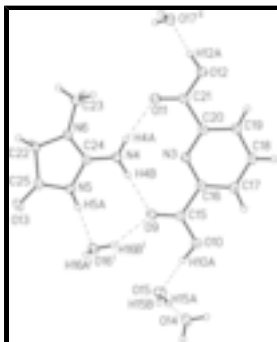
Fig. 2. Details of the hydrogen bonding between the creatinium cation, the neutral pydcH 2 molecule and the uncoordinated water molecules. Symmetry codes: (i) x, 1 + y, z , (ii) 1 - x, 1 - y, -z .
