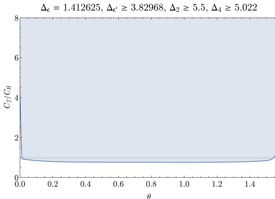
Figure 14. Lower bound on C_T as a function of \theta assuming known low-lying gaps in the parity-even spectrum in the 3d Ising CFT.
