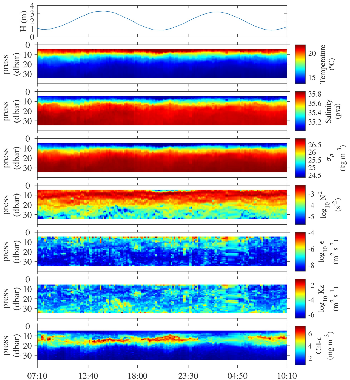
Figure 5. Vertical distribution of temperature, salinity, potential density ( \sigma_{\theta} ), decimal logarithm of buoyancy frequency squared ( N^2 ), decimal logarithm of dissipation rate of turbulent kinetic energy ( \epsilon ), decimal logarithm of vertical diffusivity ( Kz ), and chlorophyll-a fluorescence derived from the microstructure profiler during the sampling period (5–6 August 2013). Tidal height is represented at the top. Horizontal scale corresponds to Coordinated Universal Time (UTC); local time was UTC+2.
