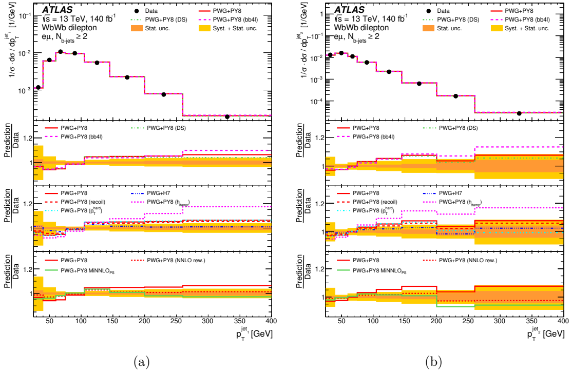
Figure 10. Relative differential cross-section measurement as a function of the (a) p_T^{\text{jet}_1} and (b) p_T^{\text{jet}_2} variables. The cross-section is unfolded to particle-level in the fiducial phase space. The measurement is compared with predictions provided by POWHEG+PYTHIA 8 with different schemes for computing the t\bar{t}/tW interference, with predictions obtained with different NLO+PS MC generators and predictions where the t\bar{t} component is simulated with an NNLO+PS MC generator or corrected to NNLO. The lower panels show the ratios of the predictions to the data with the bands showing the statistical and total uncertainties in the data. The nominal POWHEG+PYTHIA 8 prediction is included in all ratio panels.
