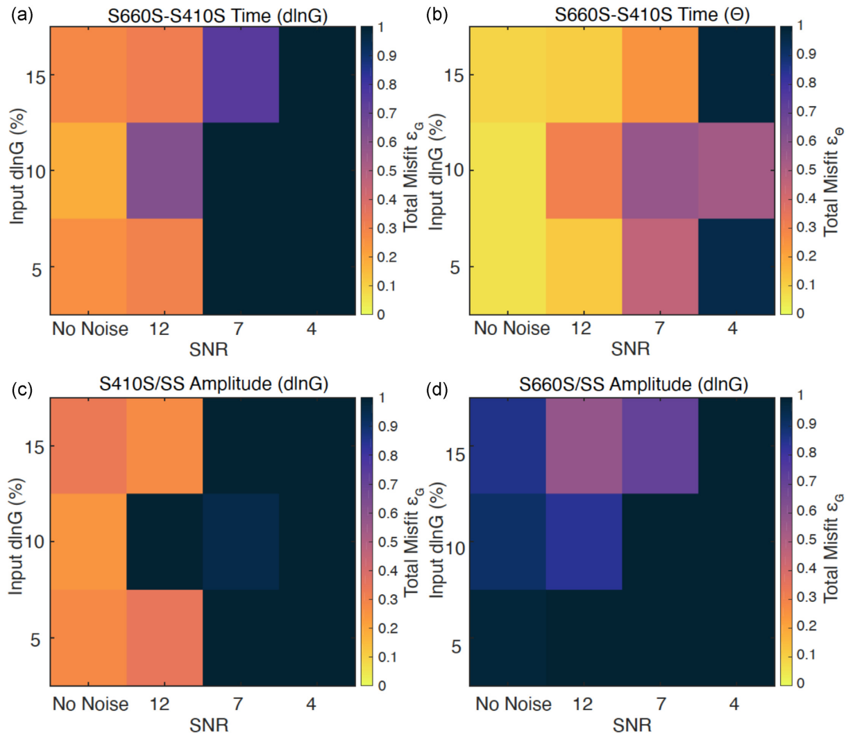
Figure 13. Detectability matrix for the Japan subduction zone using a realistic source–receiver geometry. The (a) \text{dlnG} and (b) \Theta detectability matrix for S660S–S410S time. The \text{dlnG} detectability matrix for (c) S410S/SS amplitude and (d) S660S/SS amplitude.
