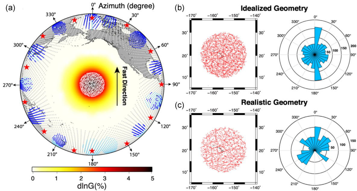
Figure 2. (a) Source–receiver geometry for the model in the central Pacific region. The red stars denote the earthquake sources. The input fast direction is due north ( 0^\circ ). The triangles represent all the stations: the light blue + dark blue stations are the ones used for the idealized geometry; the dark blue stations only are the ones used for the realistic geometry; the grey stations are the unused ones. The white points in the centre are the SS bounce points with a bin radius of 10^\circ ( \sim 1100 km). (b) The SS bounce points in the idealized geometry (left-hand panel) and their azimuthal distribution (right-hand panel). The orientations of the red sticks (left-hand panel) represent the azimuths of the SS bounce points. (c) The SS bounce points in the realistic geometry (left-hand panel) and their azimuthal distribution of the bounce points (right-hand panel) which mimics the azimuthal coverage of data in this region.
