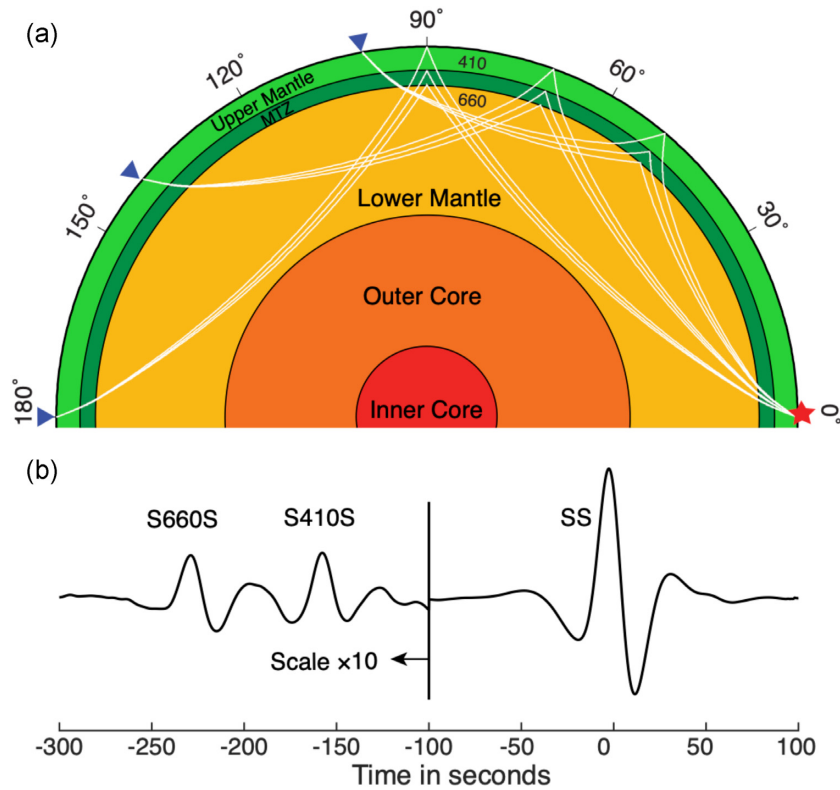
Figure 1. (a) Ray paths of SS phase and SS precursors at the epicentral distances of 100^\circ , 140^\circ and 180^\circ . The red star and blue triangles represent the source and receivers, respectively. (b) An example of stacked waveform of SS phase and SS precursors. The amplitudes of S410S and S660S are amplified by 10 times to facilitate comparisons with the SS phase.
