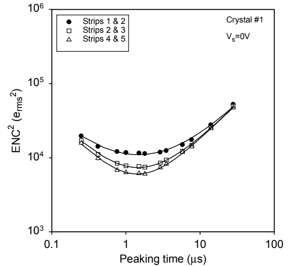
Fig. 8. Measured \text{ENC}^2 versus peaking time for crystal #1 with different pairs of strips and V_s=0\text{V} .
