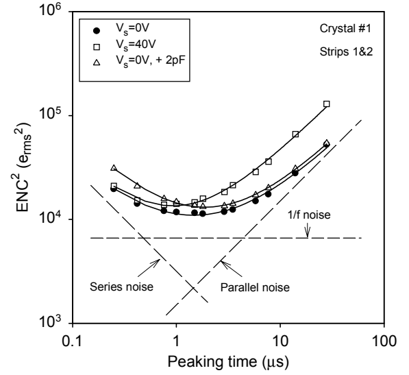
Fig. 7. Measured \text{ENC}^2 versus peaking time for crystal #1 with strips 1 and 2 connected. The dashed lines are the noise components obtained by fitting to the data for the case of V_s=0\text{V} with no capacitance added.
