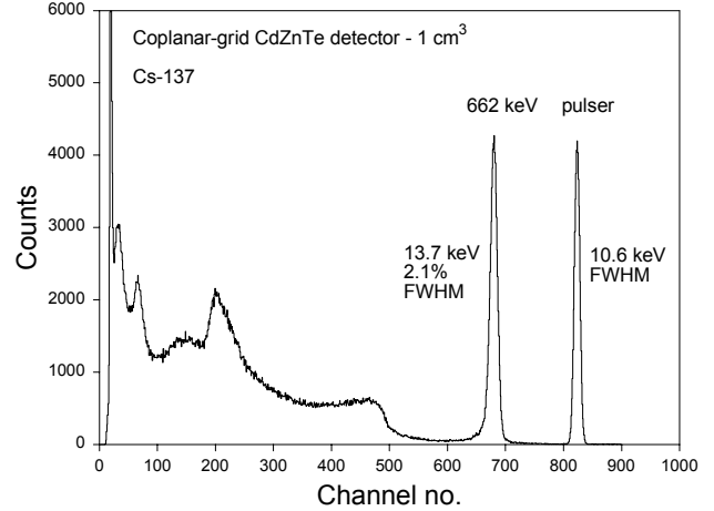
Fig. 1. A spectrum obtained from a Cs-137 gamma-ray source using a 1\text{-cm}^3 coplanar-grid CdZnTe detector.
