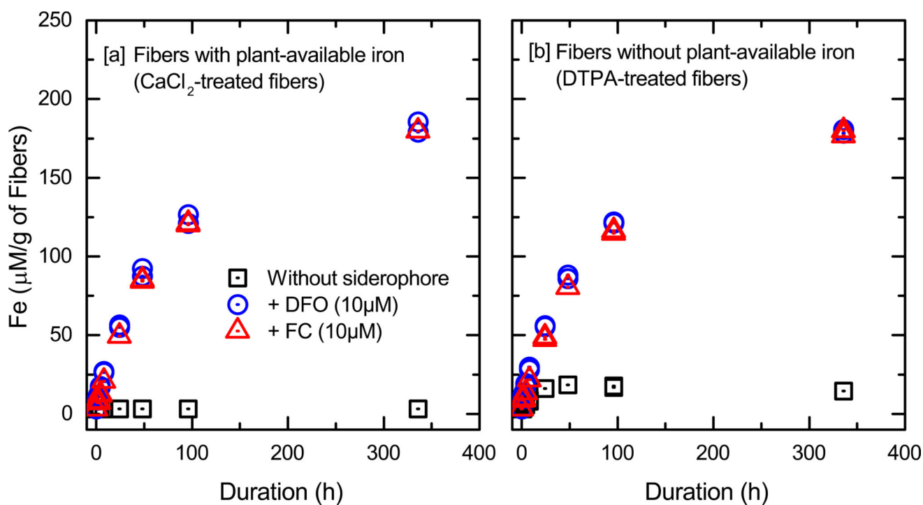
Figure 3. Removal of iron by the bacterial (DFO) and fungal (FC) siderophore from fiber (a) with plant-available iron ( \text{CaCl}_2 -treated) or (b) without plant-available iron (DTPA-treated). Each treatment was carried out in duplicate batches.
