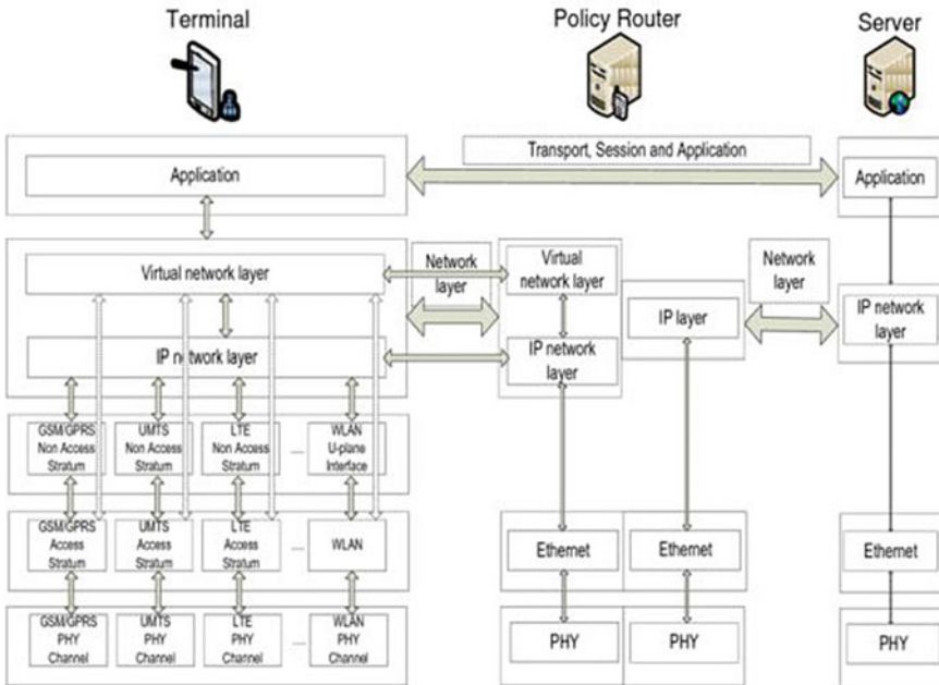
Fig. 3.3 Shows communication between client applications and server
