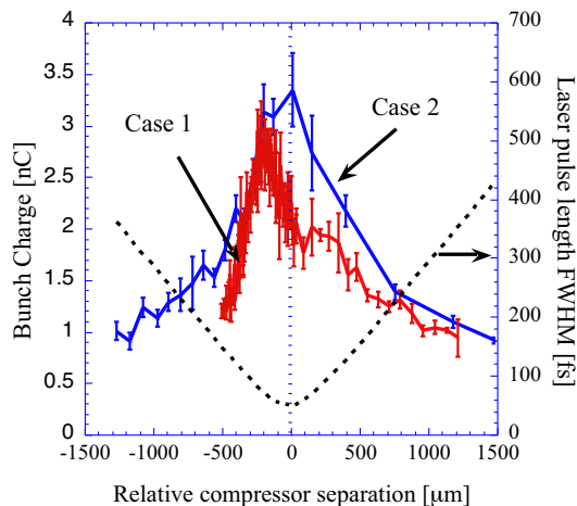
FIG. 3: Electron yield for Cases 1 and 2 and pulse duration (dashed line) vs. compressor setting. Clear asymmetry in electron yield is observed vs. compressor setting for Case 1. The energy was \sim 460 mJ/pulse and the duration \geq 50 fs.
