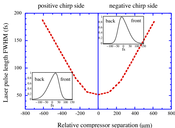
FIG. 1: Pulse duration from SSA (dashed line) vs. compressor setting and representative pulse shapes for 70-80 fs pulses. The insets show the laser pulse envelope ( I(t)/I_0 ) at two relative compressor separations corresponding to positively and negatively skewed pulses ( b = \pm 0.6 ) of duration ( \tau_{\text{FWHM}} = 76 fs).
