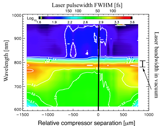
FIG. 2: Forward laser spectra vs. compressor setting. The energy was \sim 460 mJ/pulse and the duration \geq 50 fs. The laser was focused on the gas jet upstream edge.
