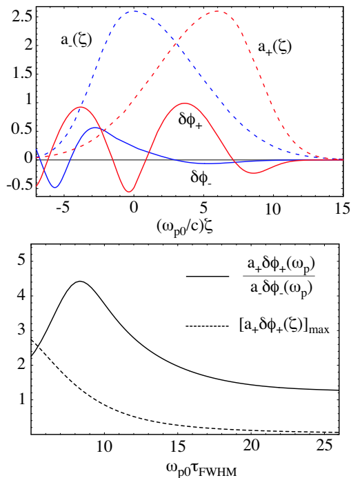
FIG. 4: (a) Plasma wave potential \delta\phi_{\pm} (solid curves) excited by pulse envelope a_{\pm}(\zeta) (dashed curves) for positive (red curves) and negative (blue curves) skewed pulses with \omega_{p0}\tau_{FWHM} = 6 for 2 \times 10^{18} cm ^{-3} density (gas jet ramp). (b) Solid curve is the ratio of the Fourier components (evaluated for \omega_p at peak intensity) of the RFS seed for ( a_{\pm}\delta\phi_{\pm} ) with pulse shapes of (a) as a function of density. Dashed curve is the maximum of [a_{\pm}\delta\phi_{\pm}(\zeta)]_{\max} .
