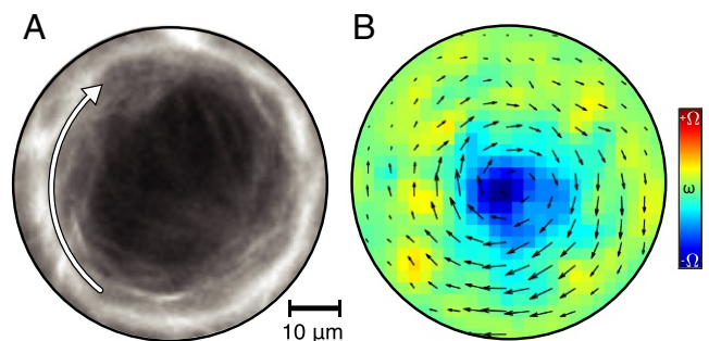
Fig. 4. Active nematics in strong confinement. (A) Circulating fluorescently labeled microtubules confined to a 60\text{-}\mu\text{m} -diameter disk (Movie S4). (B) Time-averaged (25 s) flow and vorticity fields (vorticity scale \Omega = \pm 0.19 \text{ s}^{-1} ).
