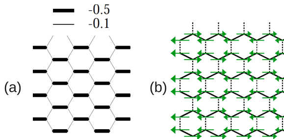
FIG. 2: (color online) (a) The ground state on the XC8 cylinder at J_2 = 0.5 , showing strong dimer correlations aligned horizontally. We call this state a dimer state. (b) The ground state on YC6 cylinder at J_2 = 0.5 . It has xy -plane collinear magnetic order, with antiferromagnetic chains along the horizontal zigzag direction together with ferromagnetic first-neighbor correlations between these zigzag chains.
