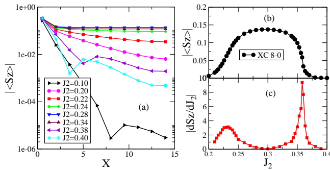
FIG. 3: (Color line) (a) Local magnetization |\langle S_z \rangle| versus distance from the end of an XC8 cylinder for various J_2 values. (b) The magnetization at the cylinder center versus J_2 . (c) The derivative of the central |\langle S_z \rangle| versus J_2 . The peaks of the derivative at J_2 = 0.23 and 0.36 indicate the two phase transition points.
