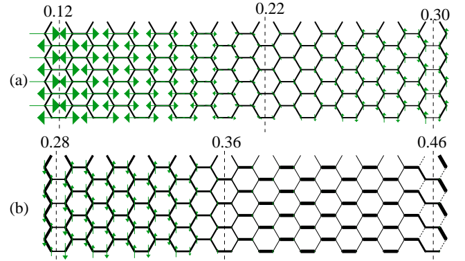
FIG. 1: (color online) (a) Local magnetic moments for an XC8 cylinder with J_2 varying along the length of the cylinder. The dashed lines show the locations of particular J_2 values. In (a), we show a cylinder with J_2 varying from 0.12 to 0.30. For J_2 \sim 0.22 , the xy -plane Neel order rotates to z -direction Ising order. In (b), J_2 is varied from 0.28 to 0.46. The second phase transition point is located at J_2 \sim 0.36 .
