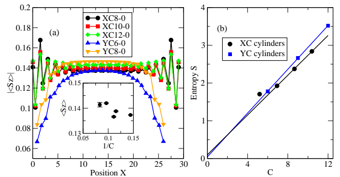
FIG. 4: (color online) (a) The absolute value of the local magnetization |\langle S_z \rangle| for various XC and YC cylinders versus distance along the cylinder. The inset shows the extrapolated magnetization (extrapolated versus the truncation error) at the cylinder center, with error bars, versus the inverse of cylinder circumference C . (b) The entanglement entropy versus circumference for XC and YC cylinders in the intermediate Ising ordered phase at J_2 = 0.3 . The intercepts are consistent with zero.
