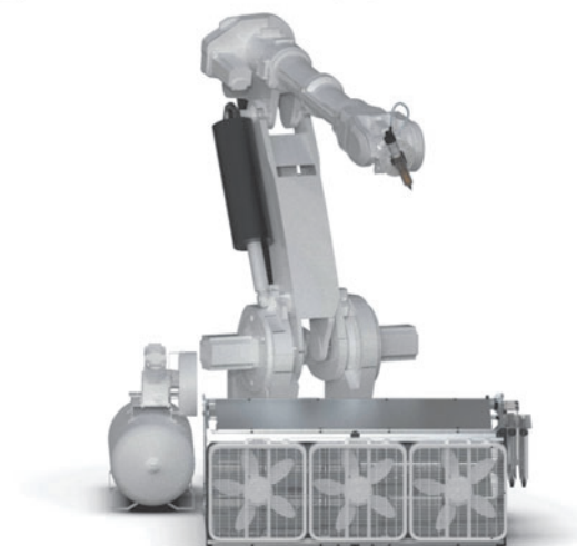
FIG. 1. Hardware specifications for a numerically controlled system for sequential multimaterial additive manufacturing. The extruder consists of a removable cartridge with interchangeable nozzles inserted into a holster. Z-axis movement is controlled via a linear actuator, while pneumatic extrusion is driven by compressed air with pressure regulated by a digital controller (A). The system can be affixed to a 6-axis industrial robot for high-precision applications (B) or to a CNC gantry with 3-axes of travel (C). In both systems, extrusion-nozzle diameter and pneumatic pressure can be adapted according to the viscosity of extruded hydrogels. A fan array can be used to accelerate hydrogel drying.
