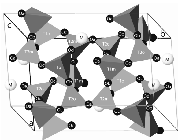
FIGURE 1. Three-dimensional illustration of an albite (An0) unit cell; andesine (An50) and anorthite (An100) unit cells are similar but twice the length in c . T-sites (gray) are most often occupied by Al or Si, and M-sites (white) are mostly occupied by Na or Ca in plagioclase feldspars. Oxygen sites are black. The unit cell is outlined with thin lines, and axes a , b , and c are in thick black.
