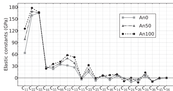
FIGURE 5. Comparison of computed An0 Model 1, An50 Model 1, and An100 elastic constants from Table 1.
