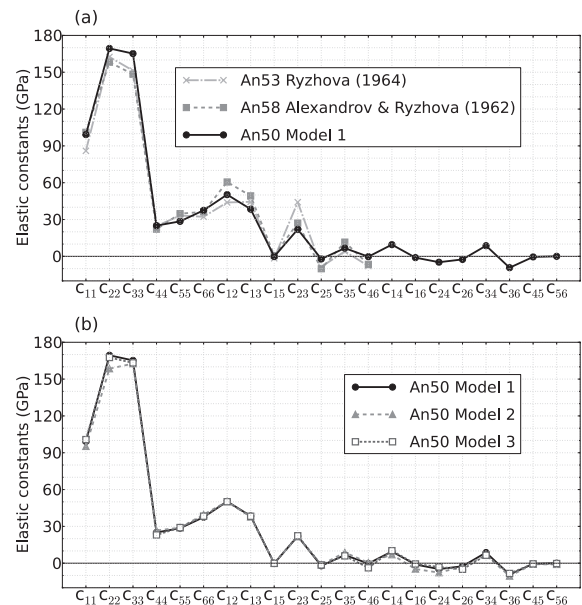
FIGURE 4. Comparison of An50 constants from Table 1. (a) Our Model 1 results are plotted with experimental results from Ryzhova (1964) and Alexandrov and Ryzhova (1962). (b) Our calculated An50 models plotted together. An50 Model 3 overlaps An50 Model 1 for most C_{ij} .
