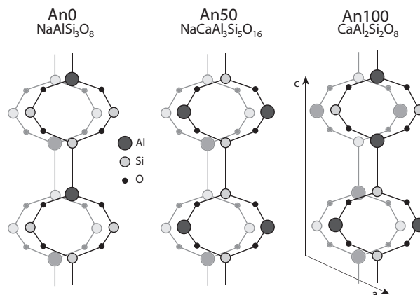
FIGURE 2. Simple schematic showing Al positions in tetrahedral rings as viewed down the b -axis in An0 Model 1, An50 Model 1, and An100. Larger dark gray circles represent tetrahedra occupied by Al, smaller light gray circles represent tetrahedra occupied by Si, and small black circles represent O atoms.
