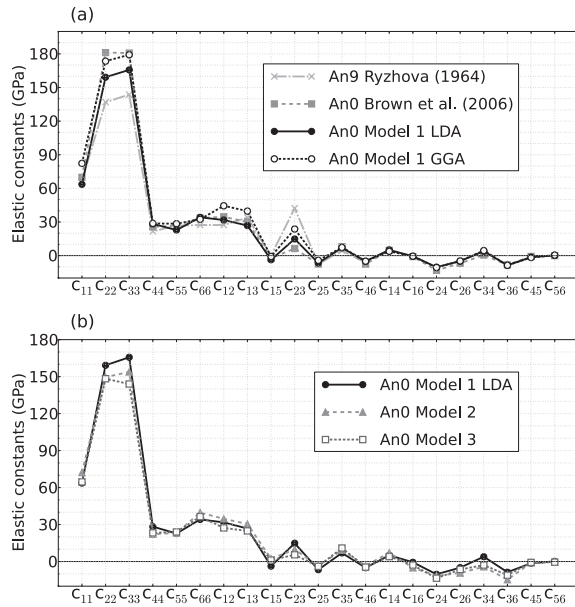
FIGURE 3. Comparison of An0 elastic constants from Table 1. (a) Our Model 1 results calculated with LDA and GGA are plotted with elastic constants measured by Ryzhova (1964) and Brown et al. (2006). (b) Results for our three An0 models.
