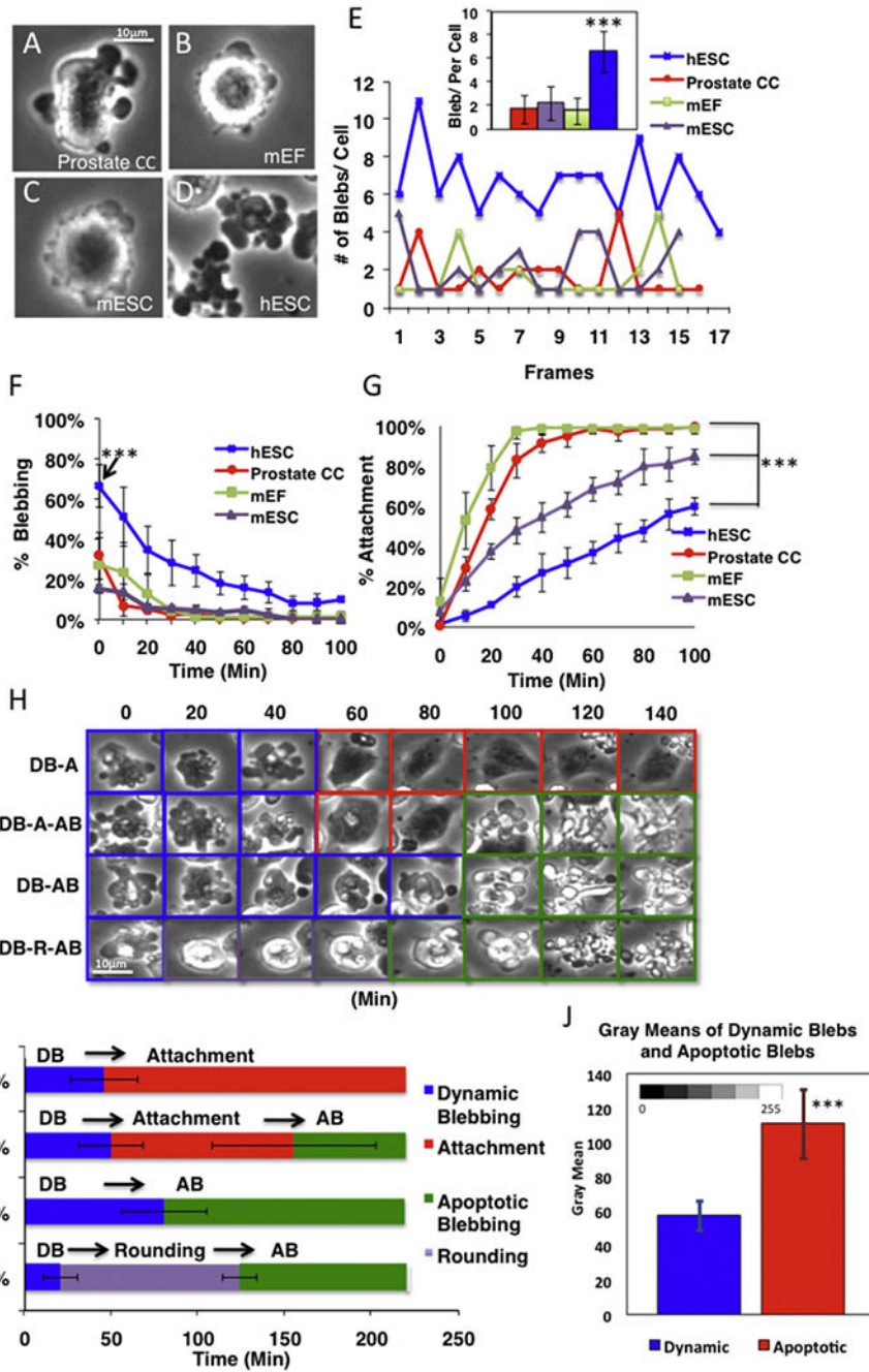
Fig. 1. Comparison of dynamic blebbing in four cell types. All cell types produced dynamic blebs: (A) human prostate cancer cell (HU145), (B) mouse embryonic fibroblast (mEF), (C) mouse embryonic stem cell (mESC), and (D) human embryonic stem cell (hESC). (E) Number of blebs/cell in different cell types in each frame before attachment. One of three independent experiments is shown. The insert shows the number of blebs/cell averaged over all frames in all three experiments. The number of blebs/cell was significantly higher in hESC than in the other cell types by one-way ANOVA. (F, G) The percentage of blebbing cells (F) and
