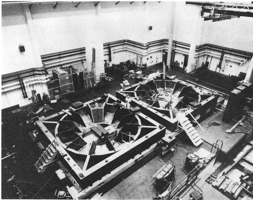
Fig. 22. The iron framework into which the hadron calorimeter chambers will be placed.
