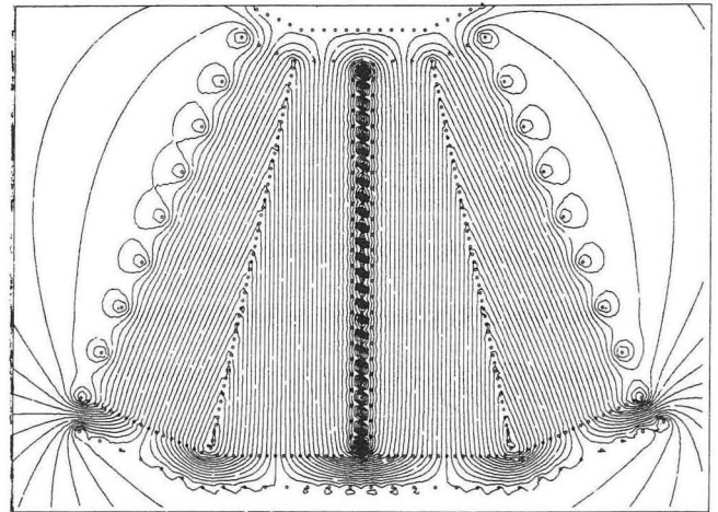
Fig. 19. The central region shows a possible design of a sector of the vertex chamber. Two adjacent half sectors are represented on either side. The lines drawn are equipotentials.
