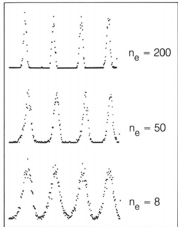
Fig. 29. Results of several scans of the electron source ( 300\mu\text{m} intervals) with varying numbers of electrons per discharge. Each peak in the figure corresponds to values of (L - R)/A taken with the gun in one location. The top scan is with 200 electrons, the middle is with 50 electrons, and the lower scan is with 8 electrons per discharge. The loss of resolution with fewer electrons is evident.
