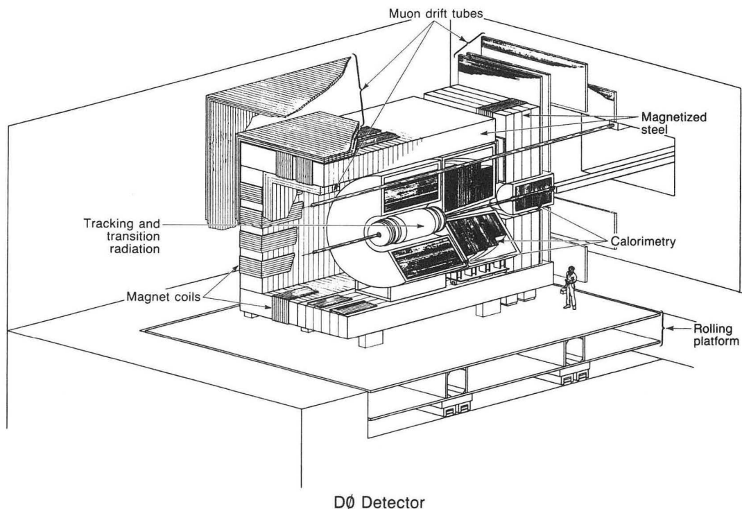
Fig. 23. Diagram of D\emptyset detector.
