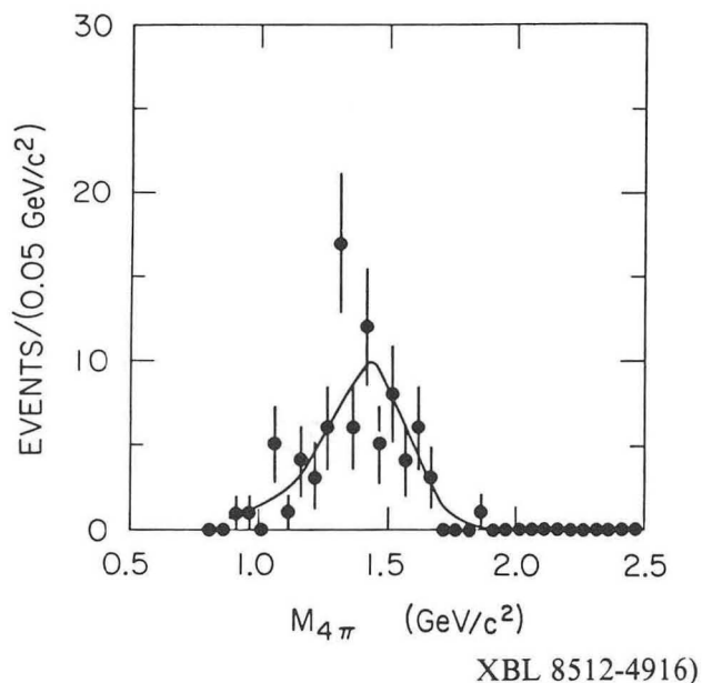
Fig. 14. Four-pion invariant mass distribution of \tau decays in the MARK II. The curve shows the expected spectrum for m(\nu_\tau) = 0 under the assumption that the four-pion \tau decay mode is dominated by the \rho' resonance.
