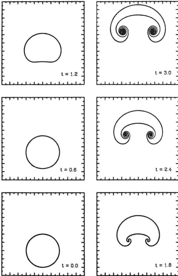
Fig. 35. Vortex method numerical simulation of the motion of a two-dimensional line thermal under the influence of gravity. Line thermals are cylindrical regions of light, less dense fluid, rising buoyantly through heavier, more dense fluid — for example, bent-over plumes issuing from smokestacks in a cross wind. The depicted curves represent the interface between lighter and heavier fluid. Individual frames give the interface location at successive times t = 0.0 to 3.0 .
