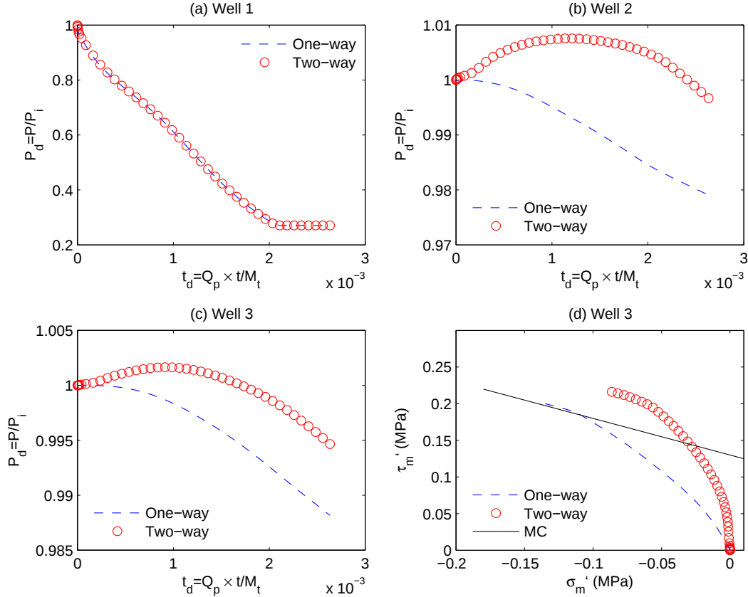
Figure 6: Comparison of the THF solutions in the low-permeability ( k_0 = k_{0,min} ) case of the 2D problem using one-way (1W) and two-way (2W) coupling formulations: (a) pressure evolution at Well 1; (b) pressure evolution at Well 2; (c) pressure evolution at Well 3; and (d) effective stress propagation at Well 3. The MC line indicates the Mohr-Coulomb model. Note that the tensile stress is positive.
