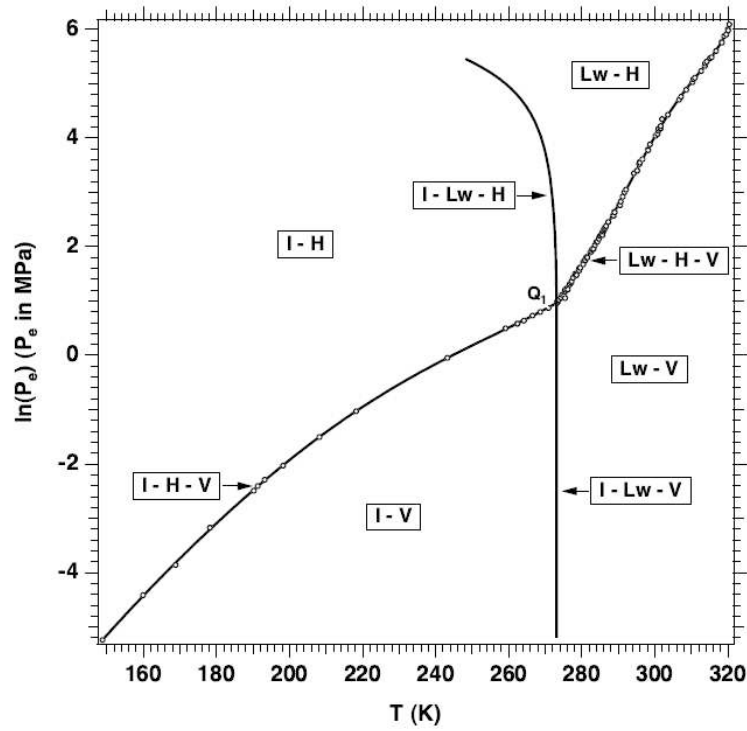
Figure 1: Pressure-temperature equilibrium relationship in the phase diagram of the water-methane-vapor-hydrate system (Moridis et al., 2008). I, V, Lw, and H indicate ice, vapor, liquid water, and hydrate phases, respectively. The dash symbol (\cdot) - (\cdot) signifies coexistence of the phases. For example, I - H means that ice and hydrate phases coexist.
