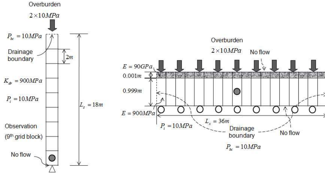
Figure 2: Configurations of the Terzaghi (a) and Mandel (b) problems. The triangles and circles at the boundaries of the two domains denote fixed displacement and rollers to constrain displacements, respectively.
