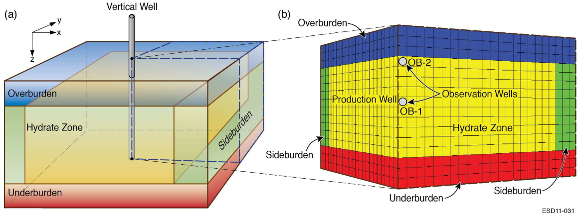
Figure 12: 3D problem of depressurization-induced gas production from a hydrate deposit using a single vertical well: (a) overall system description, depicting the overburden, underburden and sideburdens (left), and (b) description of the simulated domain, which represents only a quarter of the system because of symmetry (right). OB-1 and OB-2 denote observation wells.
