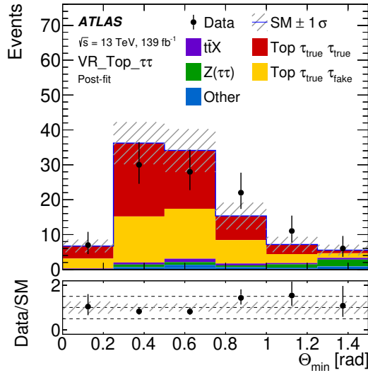
Figure 6: Kinematic distribution of the \Theta_{\min} variable in the VR_Top_ \tau\tau region. The hatched band indicates the total statistical and systematic uncertainty of the SM background. The “Other” contribution includes all the backgrounds not explicitly listed in the legend ( V +jets except Z(\tau\tau) +jets, diboson/triboson, multijet). The top-quark and Z(\tau\tau) background contributions are scaled with the normalization factors obtained from the background-only fit. The rightmost bin includes the overflow. The bottom panel shows the ratio of the observed data and the expected Standard Model background.
