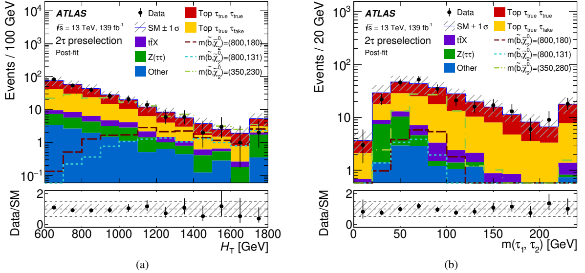
Figure 2: Kinematic distributions of data and SM background for events that pass the preselection and have at least two hadronically decaying \tau -leptons. Predictions from three signal models are also shown, where the masses m(\tilde{b}) and m(\tilde{\chi}_2^0) are given in GeV in the legend. Distributions are displayed for the (a) H_T and (b) m(\tau_1, \tau_2) variables. The hatched band indicates the total statistical and systematic uncertainty of the SM background. The “Other” contribution includes all the backgrounds not explicitly listed in the legend ( V +jets except Z(\tau\tau) +jets, diboson/triboson, multijet). The top-quark and Z(\tau\tau) background contributions are scaled with the normalization factors obtained from the background-only fit described in Section 6. The rightmost bin includes the overflow. The bottom panel shows the ratio of the observed data and the expected Standard Model background.
