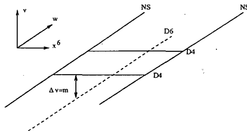
Figure 1: The Type IIA Configuration
