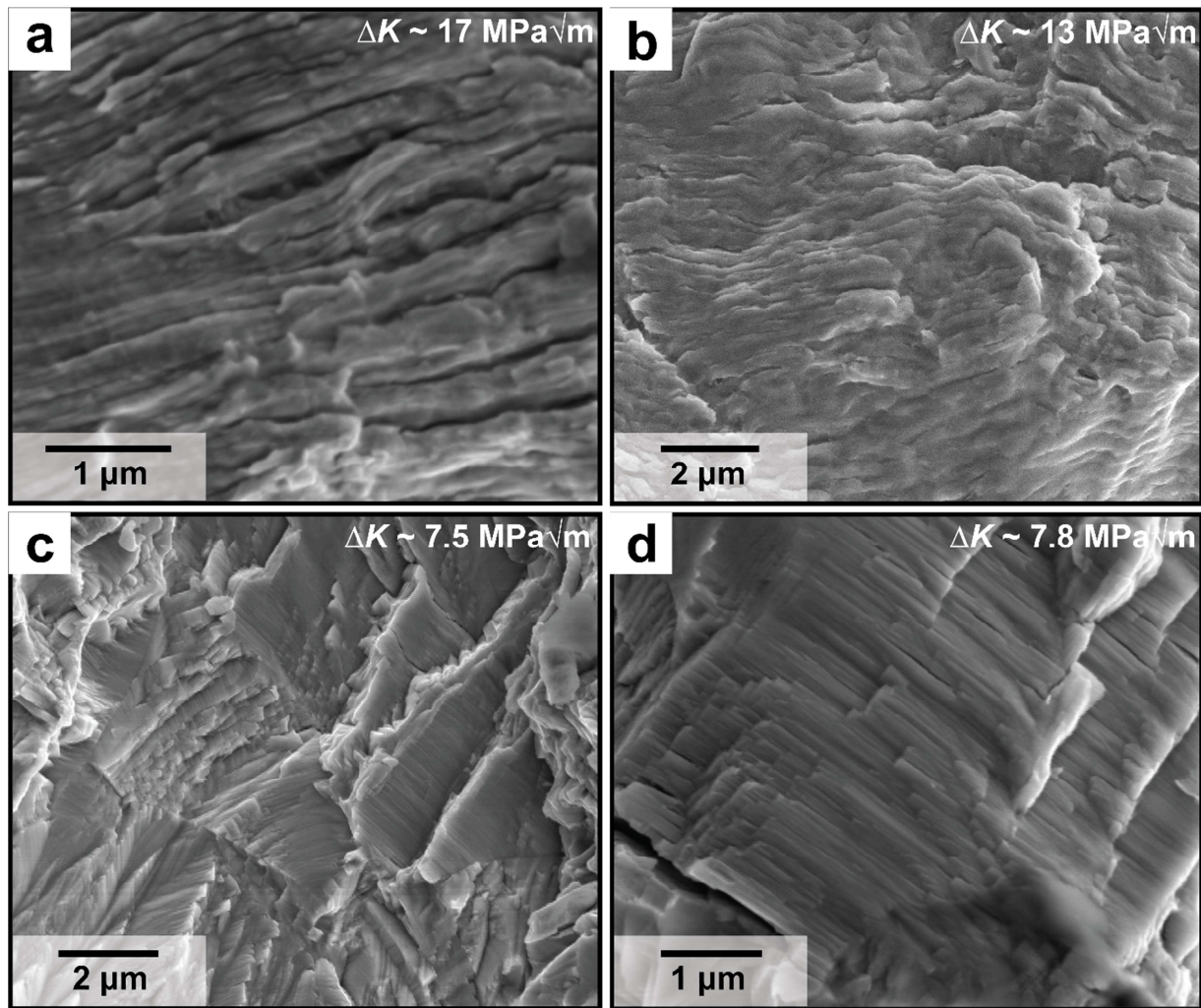
Figure 4. Striations and other microfeatures observed in higher R -ratio fatigue-crack growth testing of the CrMnFeCoNi HEA. Images (a) and (b) are 198 K tested samples at R = 0.4 and 0.7 , respectively; images (c) and (d) are 293 K at R = 0.4 and 0.7 , respectively. Striations featured prominently on the fracture surfaces of samples of all loading states, with particular prominence at higher \Delta K levels, as this corresponds to higher crack-growth rates and thus larger striation spacings. Additionally, striations were found at lower \Delta K levels at ambient temperature, and again appeared to be more prominent at the higher R -ratios.
