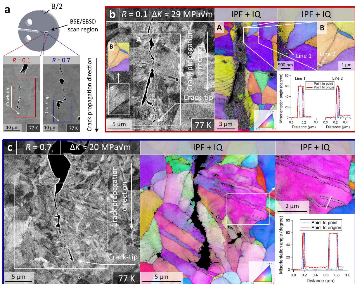
Figure 5. Deformation mechanisms in the vicinity of the crack tip in the CrMnFeCoNi high-entropy alloy (HEA) fatigue tested under R -ratios of 0.1 and 0.7 at 77 K. (a) Low-magnification secondary electron (SE) images captured in the crack-tip regions on the sliced mid-plane section of the C(T) specimen. (b) High-magnification back-scattered electron (BSE) images and electron-backscatter diffraction (EBSD) scans taken from the sample subjected to R = 0.1 with \Delta K \approx 29 \text{ MPa}\sqrt{\text{m}} ( K_{\text{max}} \approx 32 \text{ MPa}\sqrt{\text{m}} ). At higher \Delta K levels, fracture is predominately transgranular, but an intergranular faceted mode of fracture becomes more prominent as the growth rates are reduced. BSE scans reveal the formation of dislocation cells and deformation nano-twins in the wake of the propagated crack within a region of 1-3 grains. The EBSD image, which is an overlaid map of inverse pole figure (IPF) and image quality (IQ) clearly shows deformation-induced nano-twinning at 77 K. Nano-twinning is confirmed by line scans across the twin boundaries, showing the 60^\circ misorientation angle between the twin domain and the parent grain domain. (c) Corresponding BSE and EBSD images taken from the sample subjected to R = 0.7 with \Delta K \approx 20 \text{ MPa}\sqrt{\text{m}} show pronounced nano-twinning and dislocation cells formed in the wake of the propagated crack.
