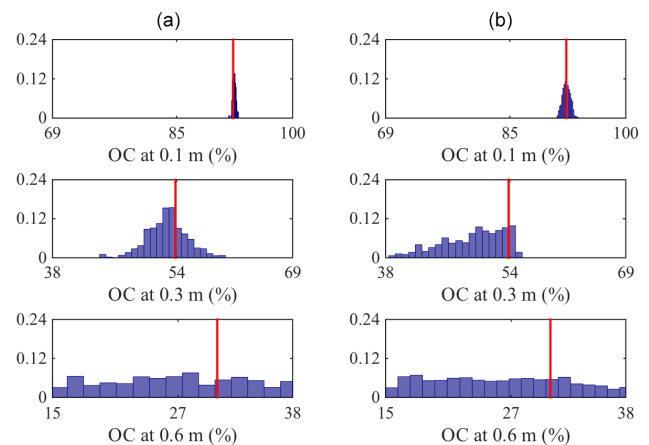
Figure 6. The a posteriori probability of the soil OC content at z = 0.1, 0.3 and 0.6 m obtained by inverting apparent resistivity data with relative measurement error of 2% (a) and 5% (b). The red lines represent the “true” OC content.
