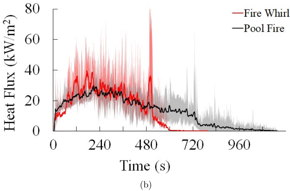
Figure 2.4: Average heat flux recorded during the burning of a) 3.5 mm thick slick ANS pool fires and fire whirls b) 11 mm thick slick ANS pool fires and fire whirls. Shaded regions represent the full range of values across the averaged tests.
