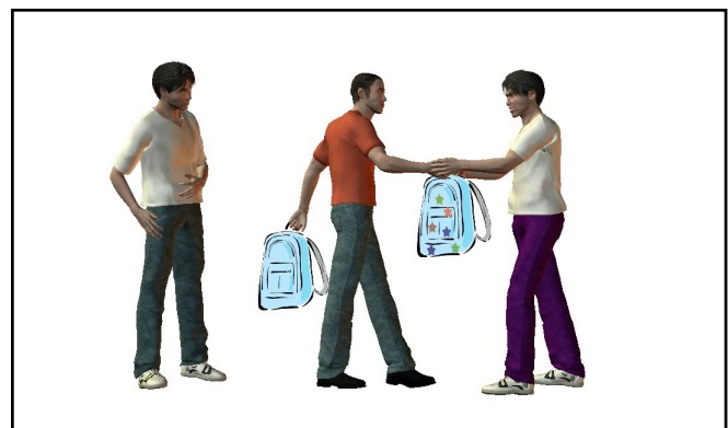
Figure 1: Still image from the animation designed to elicit contrast on both the theme and the recipient (as in “Simon gave a backpack with stars to a man with purple pants ”)
