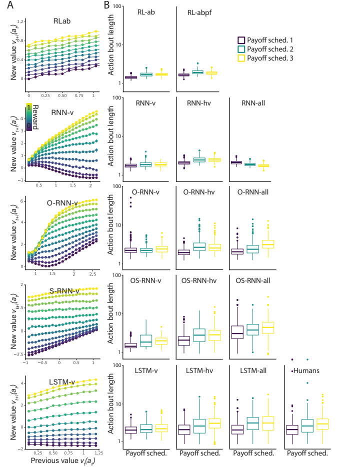
Figure 2: A) Analyzing learned learning rules. All “v models” update v(a) on each trial, using parameters and (except for RL_{\alpha\beta} ) update functions (learning rules) learned from human data. X-axes ( v_t(a_t) ) and colors ( r_t ) show function inputs, y-axes show function outputs ( v_{t+1}(a_t) ), for a full specification of the learned functions. Methods: 10,000 random input tuples were passed through each update function to obtain outputs. r_t was sampled randomly across the allowed range [0, 1] ; v_t(a_t) and s_t were sampled within 3 standard deviations of their mean along their first principal component (PC). Points indicate means, error bars standard errors of the mean, after binning data points into 0.1-sized bins based on reward magnitude. Differences in y-axis scale can be interpreted as differences in “decision temperature”. B) Assessing qualitative model fit using behavioral simulations. We used human-fitted parameters \theta to simulate artificial behavior, and subjected all (artificial and human) datasets to the same behavioral analyses. Action bout length (participants’ average numbers of subsequent identical actions) is one example behavior. Box plots show the 25th, 50th (median), and 75th percentile over participants; whiskers extend to the 1.5-fold interquartile range; remaining participants are represented by dots. Models are arranged in the same way as in Fig. 1. Qualitative model fit, i.e., similarity to human behavior (top-right), closely mirrors quantitative model fit (Fig. 1, Table 1), with similar results for behaviors other than action bout length.
