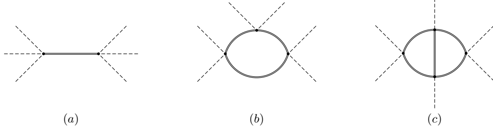
FIG. 4. Graphs contributing to \phi^6 matching from integrating out a heavy scalar \Phi . \phi is denoted by a dashed line, and \Phi by a double line.
