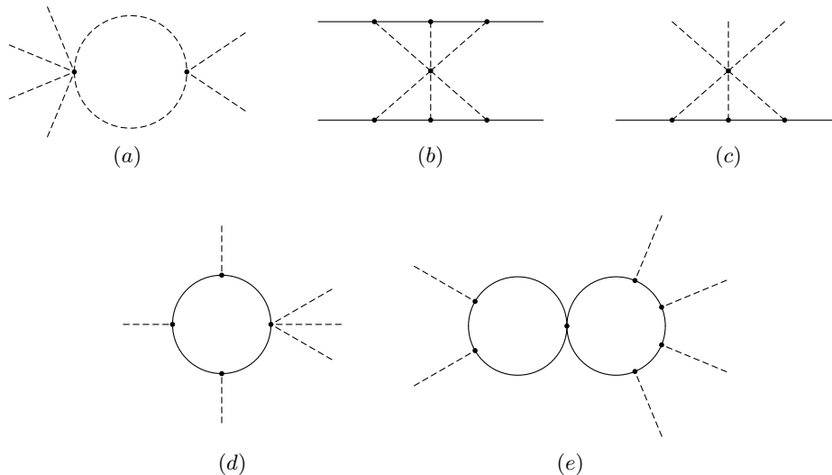
FIG. 3. A few SMEFT graphs. H is denoted by a dashed line, and \psi by a solid line.
