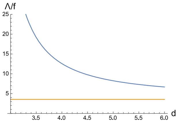
FIG. 1. Plot of \Lambda/f as a function of spacetime dimension d . The asymptotic value as d \rightarrow \infty is \sqrt{4\pi} , shown as the horizontal line.
