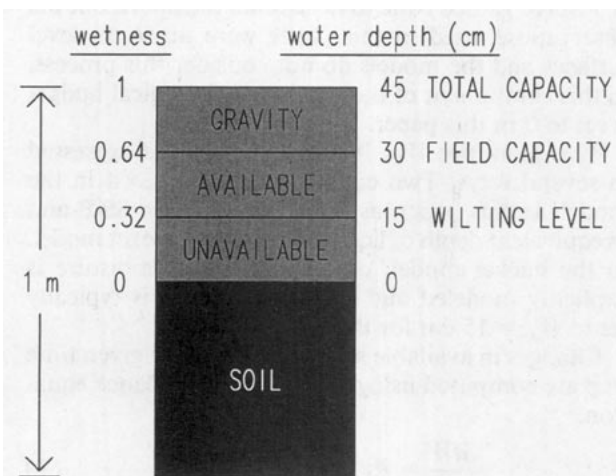
FIG. 2. Illustration of the typical contents of the top 1 m of soil, with the three water partitions. On the left are typical values of soil wetness from SSiB, and on the right, typical values of water depth from the bucket model.
