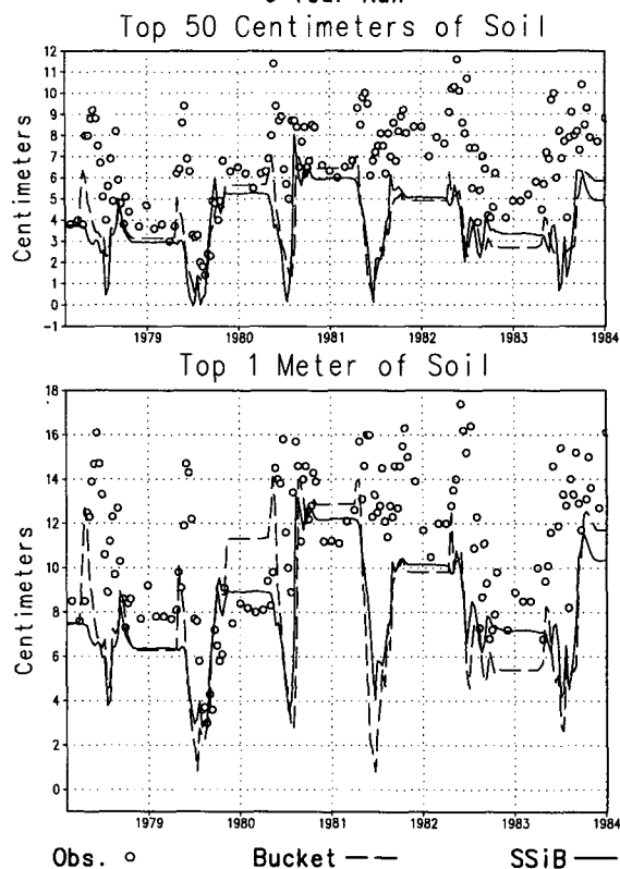
FIG. 18. Simulations and observations of available soil moisture for Tulun for 1978–1983, shown as 10-day averages. See Figs. 7 and 8 for the 1979–1983 average seasonal cycle.
