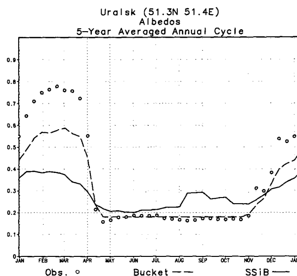
FIG. 14. Simulated and observed albedos for Uralsk simulations shown in Fig. 9, shown as 10-day averages of 5-yr average seasonal cycles.
