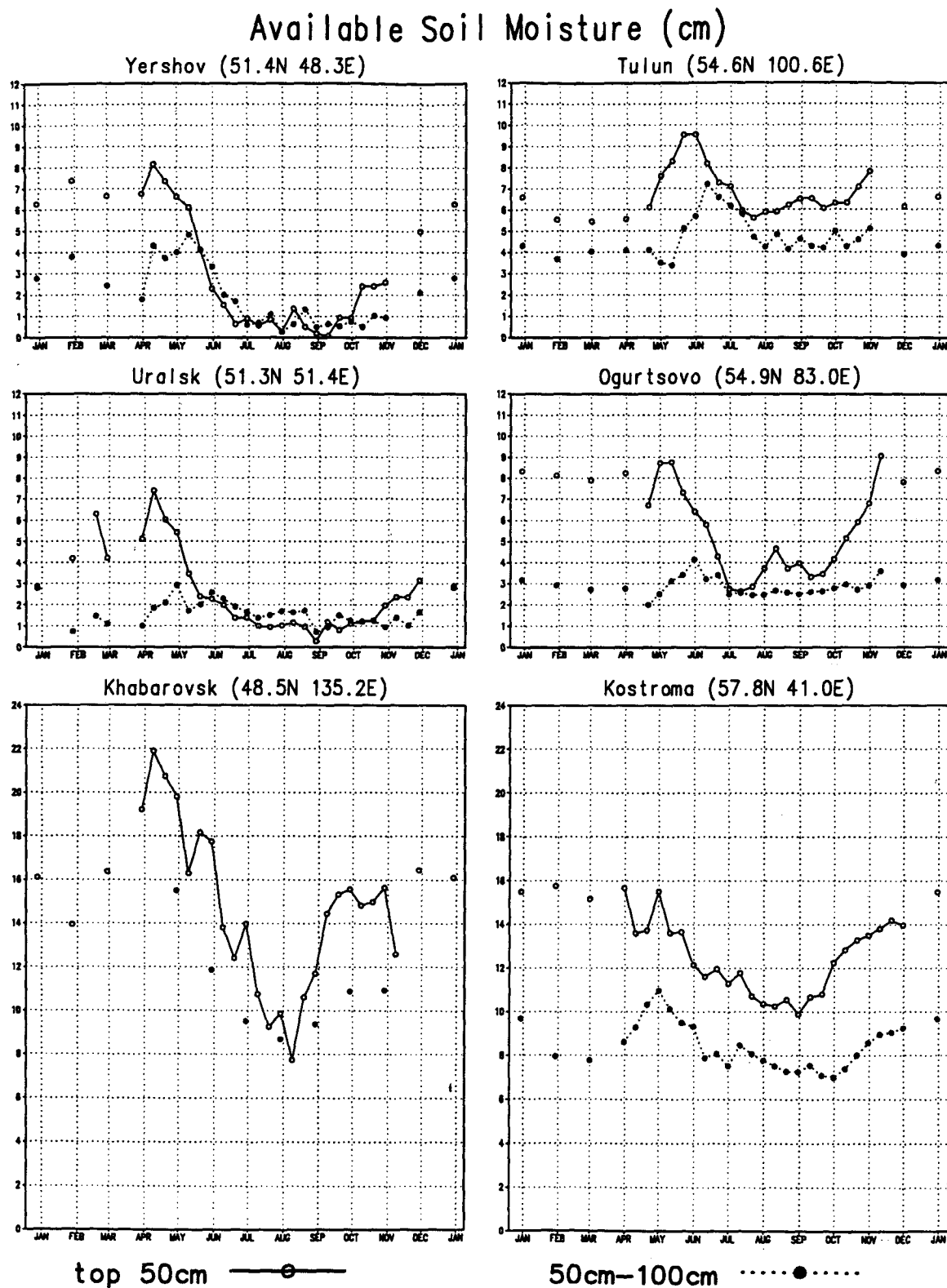
FIG. 5. The 6-yr average (1978–1983) seasonal cycle of observed available soil moisture in the top two 0.5-m layers for the six stations (Fig. 1, Table 1). The abscissa labels indicate the beginning of the months. The data points taken every 10 days during the growing season are connected with lines. The other data points represent end of the month measurements.
