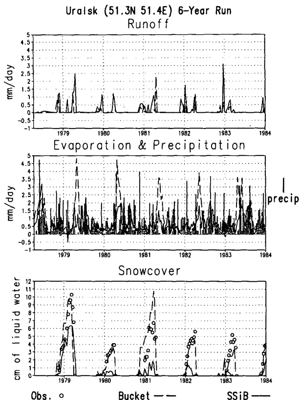
FIG. 10. Components of the hydrological budget for Uralsk simulations in Fig. 9, shown as 10-day averages. For runoff and evaporation, only simulations are available. Observed precipitation, used as forcing in the simulations, is shown. For snow cover, simulations and observations are shown.
