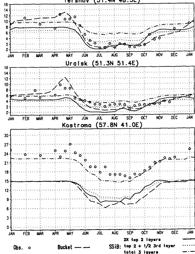
FIG. 6. Comparison of three methods of comparing 1-m SSiB results with observations and bucket results at three different stations, with results averaged over the last 5 yr of the 6-yr simulations.
