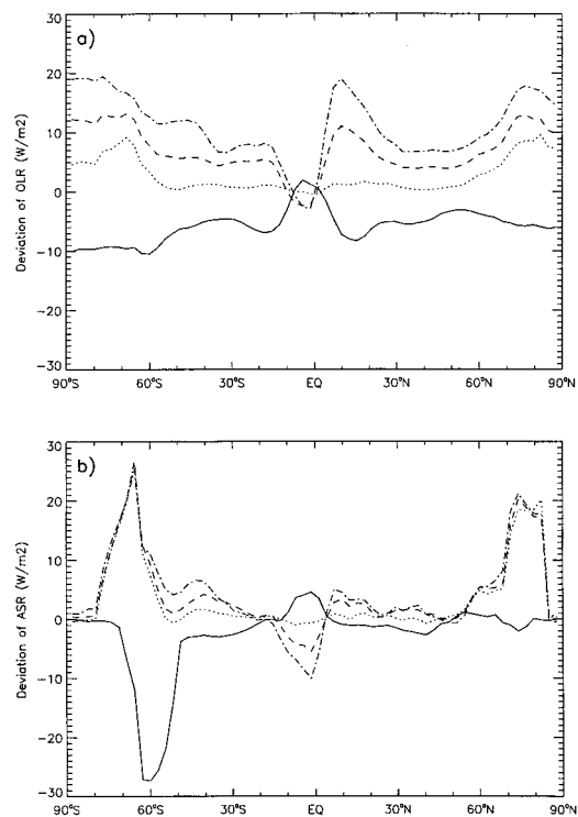
Fig. 7. Zonally averaged, annual-mean, vertical energy flux ( \text{W m}^{-2} ) at the top of the atmosphere averaged over nine years, shown as deviations from the control case (0X), as functions of latitude. -5X (solid), 1X (dotted), 5X (dashed), 9X (dot-dashed). (a) Deviations of OLR from 0X. (b) Deviations of ASR from 0X.
