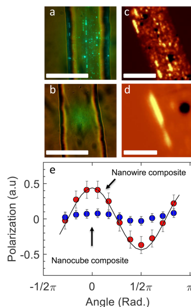
Figure 3. Polarized emission from aligned perovskite nanowires. (a) Optical microscope image of a mechanically drawn nanowire–polymer (PLMA) composite fiber. Shear forces align the high aspect ratio ( >100 ) nanowire bundles parallel to the long axis of the polymer composite fiber. The nanowires are excited with 456 nm laser light and emit green 517 nm light. (b) Nanocube–polymer composite fibers fabricated with the same conditions do not show similar alignment. Scale bar, 20 \mu\text{m} . (c) Confocal microscope image of emitted light (band-pass filter 514 \pm 10 nm) depicting the alignment of bundles inside the fiber and a close-up depicting (d) two such aligned bundles. (e) Calculated polarization ( P = \frac{I_{\parallel} - I_{\perp}}{I_{\parallel} + I_{\perp}} ) as a function of polarized analyzer angle of nanowire–polymer fiber (red) and nanocube–polymer fiber (blue) demonstrating significant polarized emission ( P_{\text{max}} = 0.44 ) in the nanowire composite parallel to the fiber axis, as compared to the nanocube composite ( P_{\text{max}} = 0.08 ).
