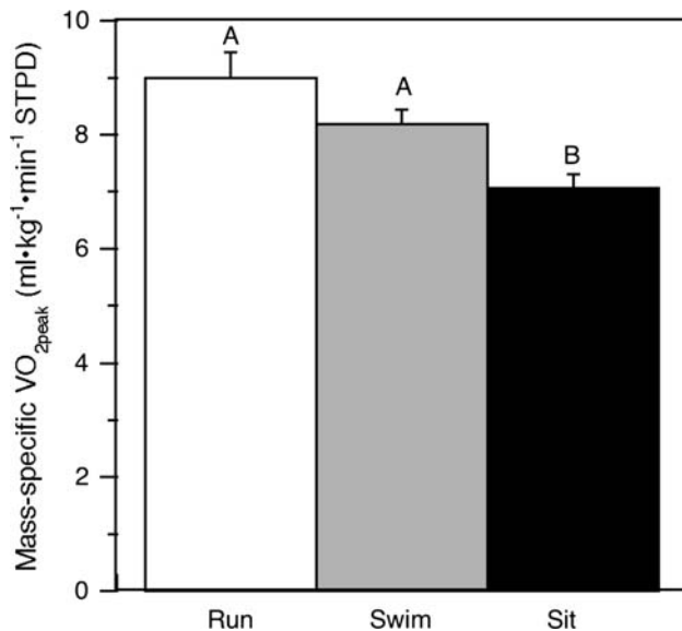
Fig. 2 Mean mass-specific peak oxygen consumption rate recorded during a graded treadmill exercise test for alligators from different exercise groups, run, swim and sedentary (sit). Run and swim groups had significantly higher \dot{V}_{O_2} peak than the sedentary (sit) group. Uppercase letters above error bars indicate significant differences between groups derived from Kruskal–Wallis rank sums test ( \alpha = 0.05 ) followed by Wilcoxon rank sums test with Bonferroni correction ( \alpha = 0.0167 ). Error bars are SE
