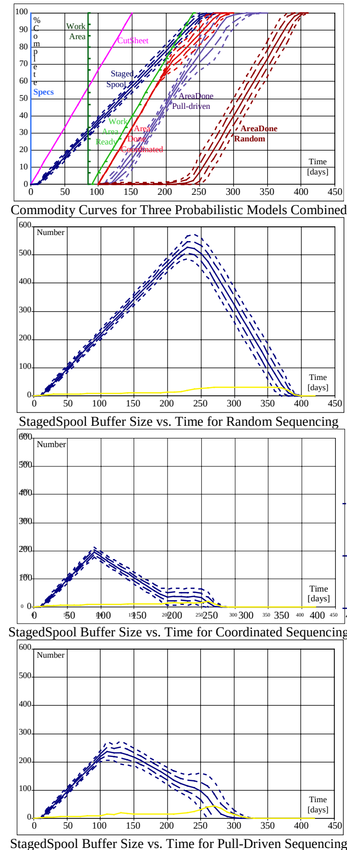
Figure 4: Simulation Output of 1,000 Iterations
