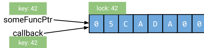
Figure 3.3: Each pointer has a key, each object has a lock.
