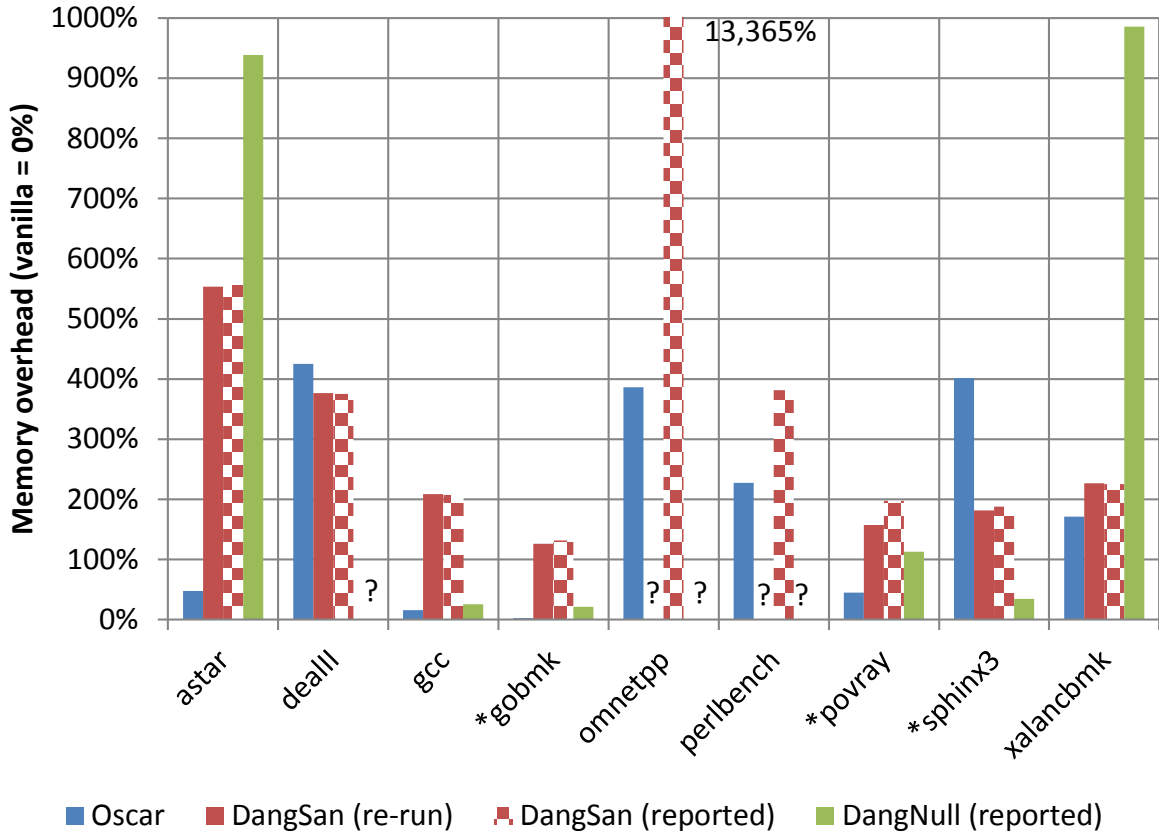
Figure 3.20: Memory overhead on CPU2006 (continued). ‘?’ indicates that DangNull did not report memory usage for dealII , omnetpp , or perlbench , and we could not re-run DangSan on the latter two.
