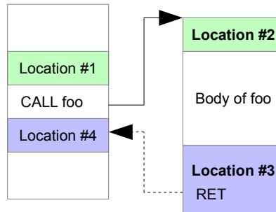
Figure 2.2: Possible locations for instrumentation.
