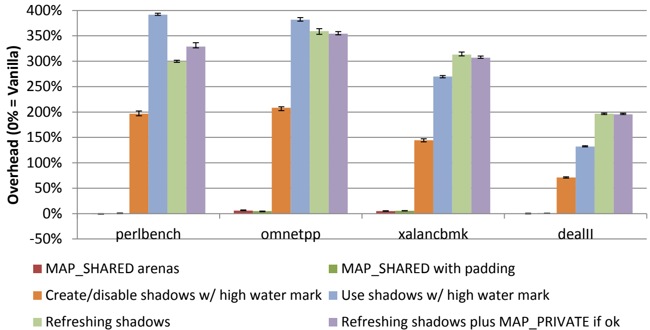
Figure 3.16: The 4 allocation-intensive benchmarks. Note that the first two columns are near zero for each benchmark.
