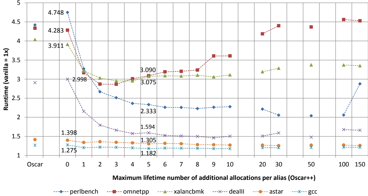
Figure 4.3: Oscar++ runtimes for the six higher-overhead non-Fortran SPEC CPU2006 benchmarks. n = maximum lifetime number of additional allocations per alias, for Oscar++.
