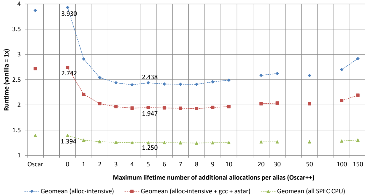
Figure 4.5: Oscar++ runtimes: geometric means. n = maximum lifetime number of additional allocations per alias, for Oscar++. The y-axis is different from previous figures.
