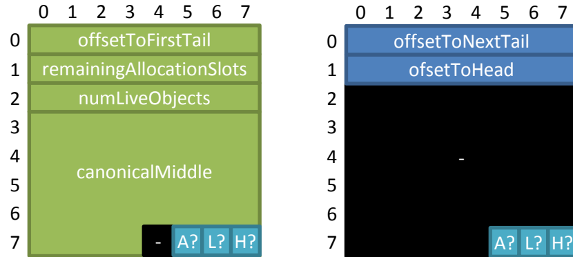
Figure 4.2: Oscar++ metadata for head (left) and tail (right) objects. A = truly aliased (see Section 4.2.3), L = live object, H = head.
