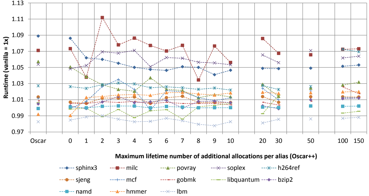
Figure 4.4: Oscar++ runtimes for the non-Fortran SPEC CPU2006 benchmarks, other than the six higher-overhead benchmarks of Figure 4.3. n = maximum lifetime number of additional allocations per alias, for Oscar++. The y-axis is different from Figure 4.3.
