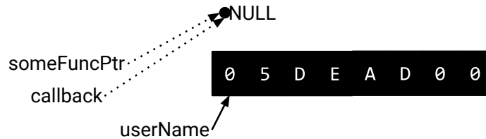
Figure 3.6: After pointer nullification (see Figure 3.1 for the ‘Before’), object space can be reused safely.
