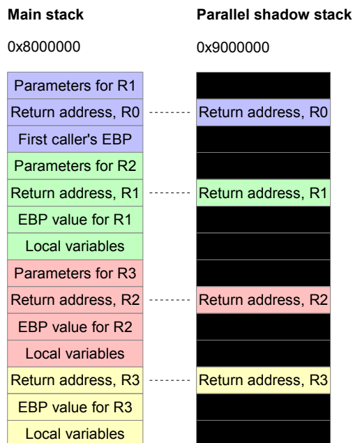
Figure 2.8: Parallel shadow stack. Rx refers to Routine #x. Compare to the traditional shadow stack of Figure 2.1.
