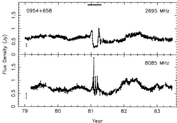
Figure 1. Original ESE observations of Fiedler et al (1987).
