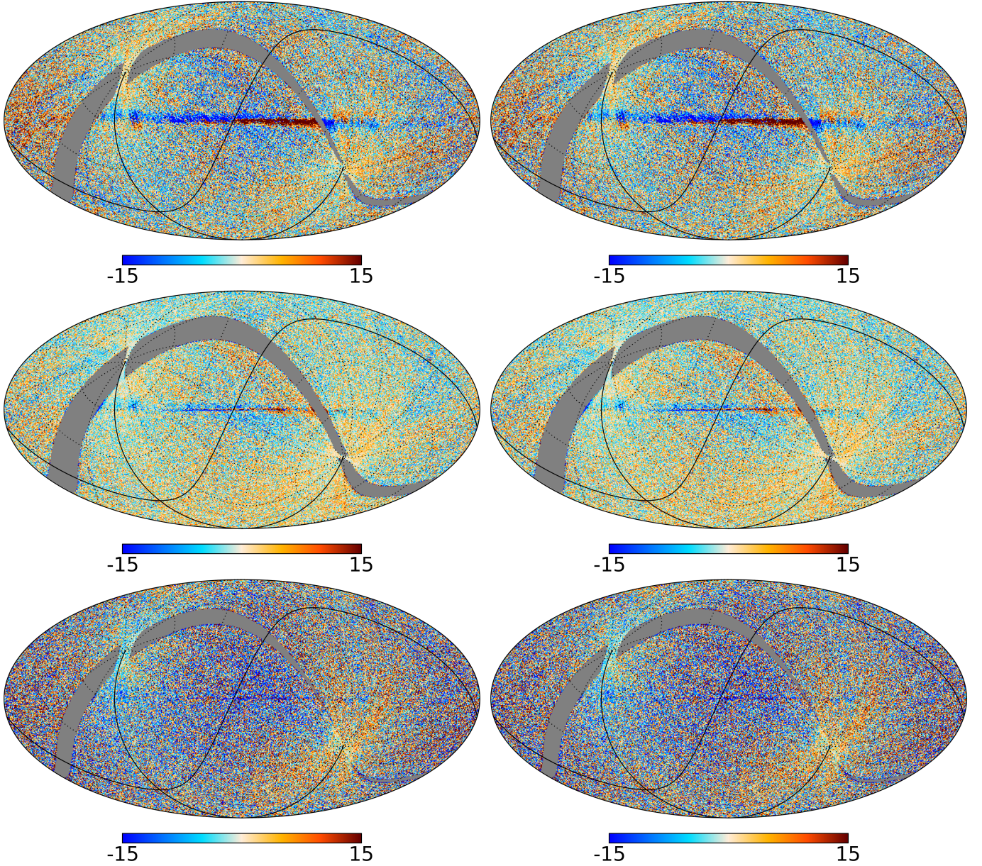
Fig. 11. Survey 2 minus Survey 1 difference maps before ( left ) and after ( right ) zodiacal emission removal. The rows, from top to bottom , are for 217, 143, and 100 GHz. All maps are in units of \mu\text{K}_{\text{CMB}} .
